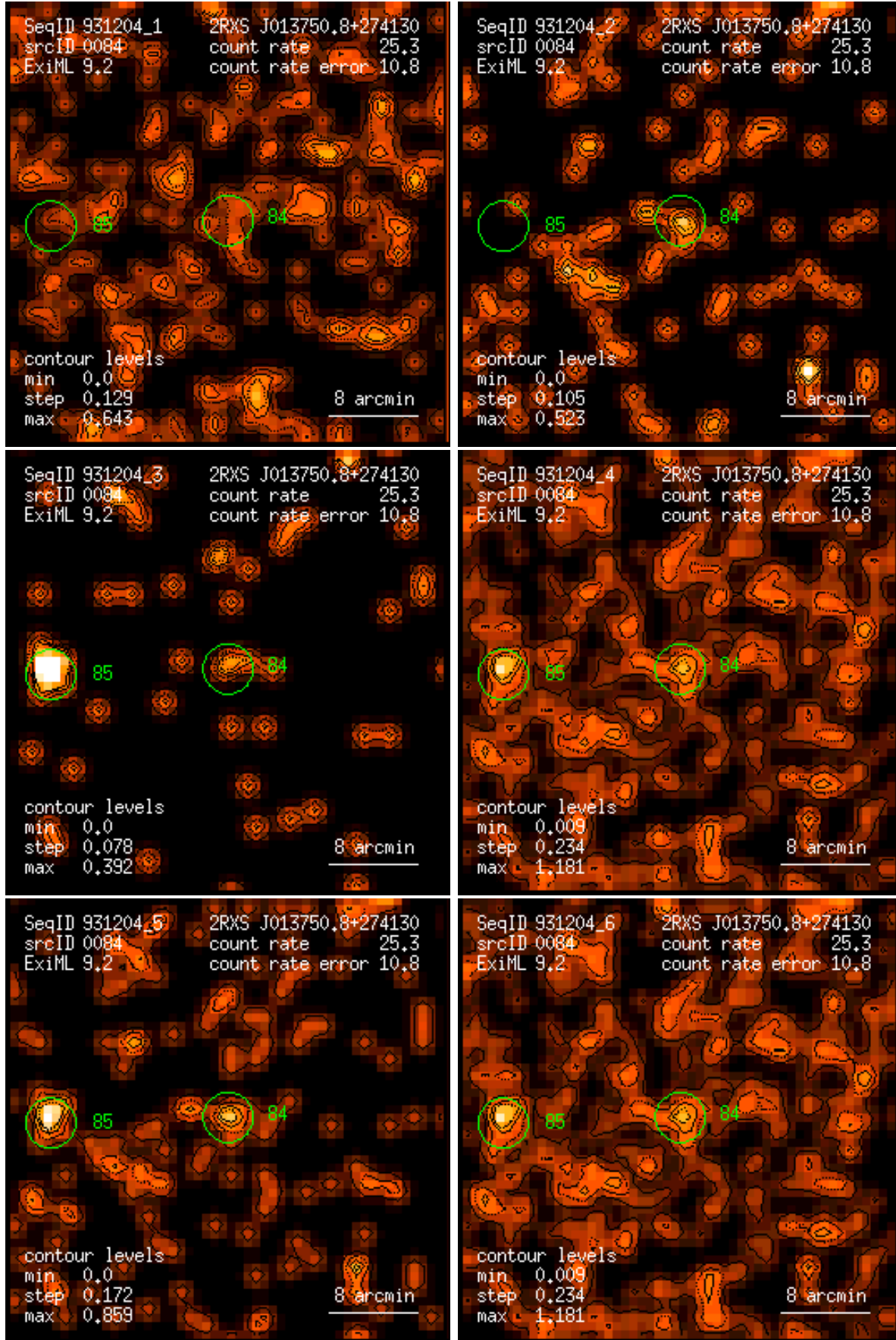
Figure 84: RASS 931204: detection 0084: band rate images, Gaussian filter: (1) PSPC channels 11 – 41, (2) 52 – 90, (3) 91 – 201, (4) 11 – 235, (5) 52 – 201, (6) 11 – 201. Broad band rates in counts/ks. Band rate contour levels in counts/ks/arcmin 2 .
