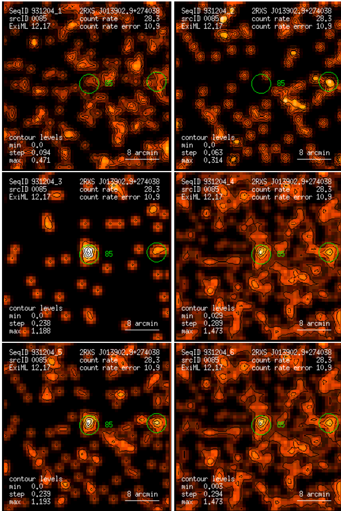
Figure 85: RASS 931204: detection 0085: band rate images, Gaussian filter: (1) PSPC channels 11 – 41, (2) 52 – 90, (3) 91 – 201, (4) 11 – 235, (5) 52 – 201, (6) 11 – 201. Broad band rates in counts/ks. Band rate contour levels in counts/ks/arcmin 2 .
