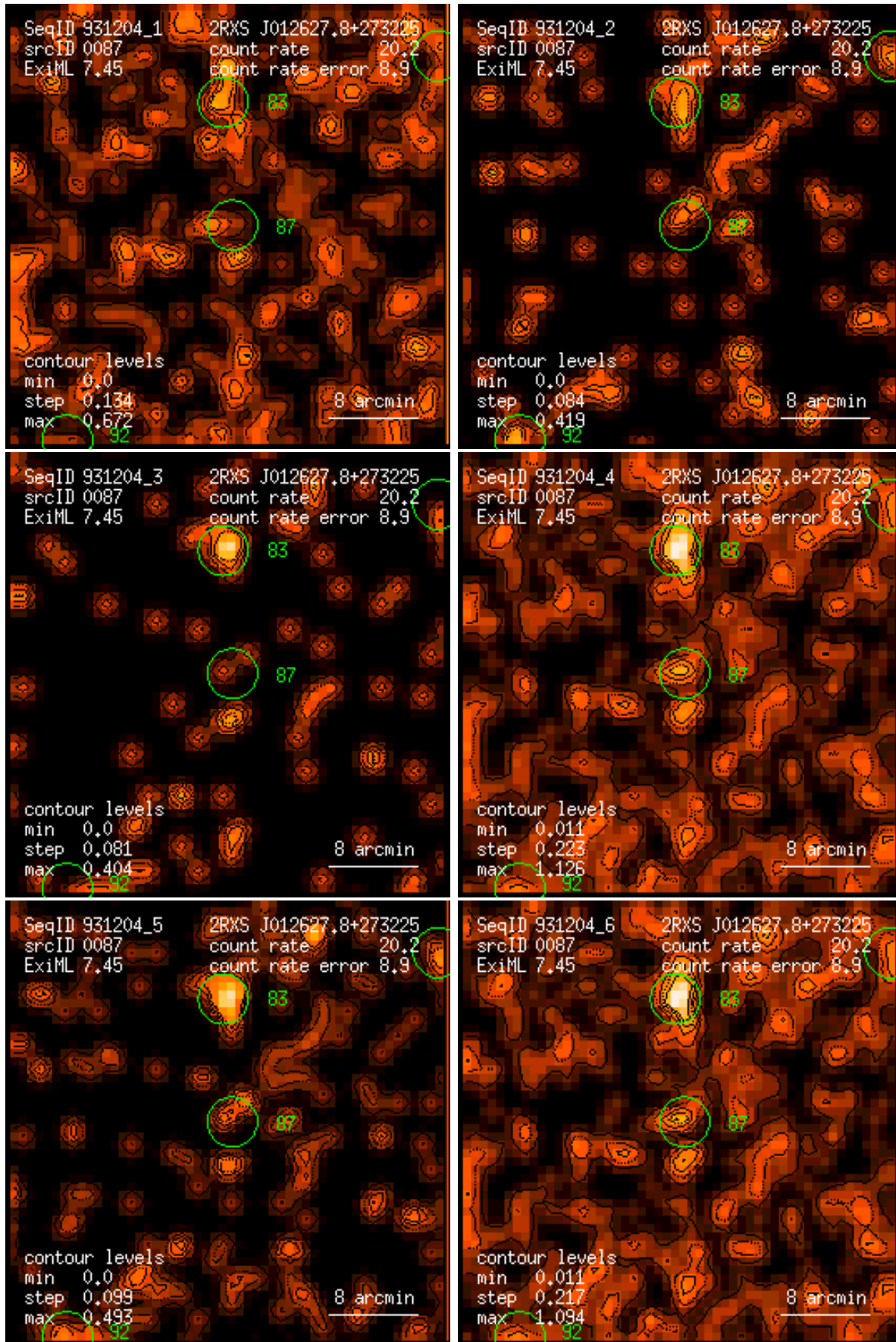
Figure 87: RASS 931204: detection 0087: band rate images, Gaussian filter: (1) PSPC channels 11 – 41, (2) 52 – 90, (3) 91 – 201, (4) 11 – 235, (5) 52 – 201, (6) 11 – 201. Broad band rates in counts/ks. Band rate contour levels in counts/ks/arcmin 2 .
