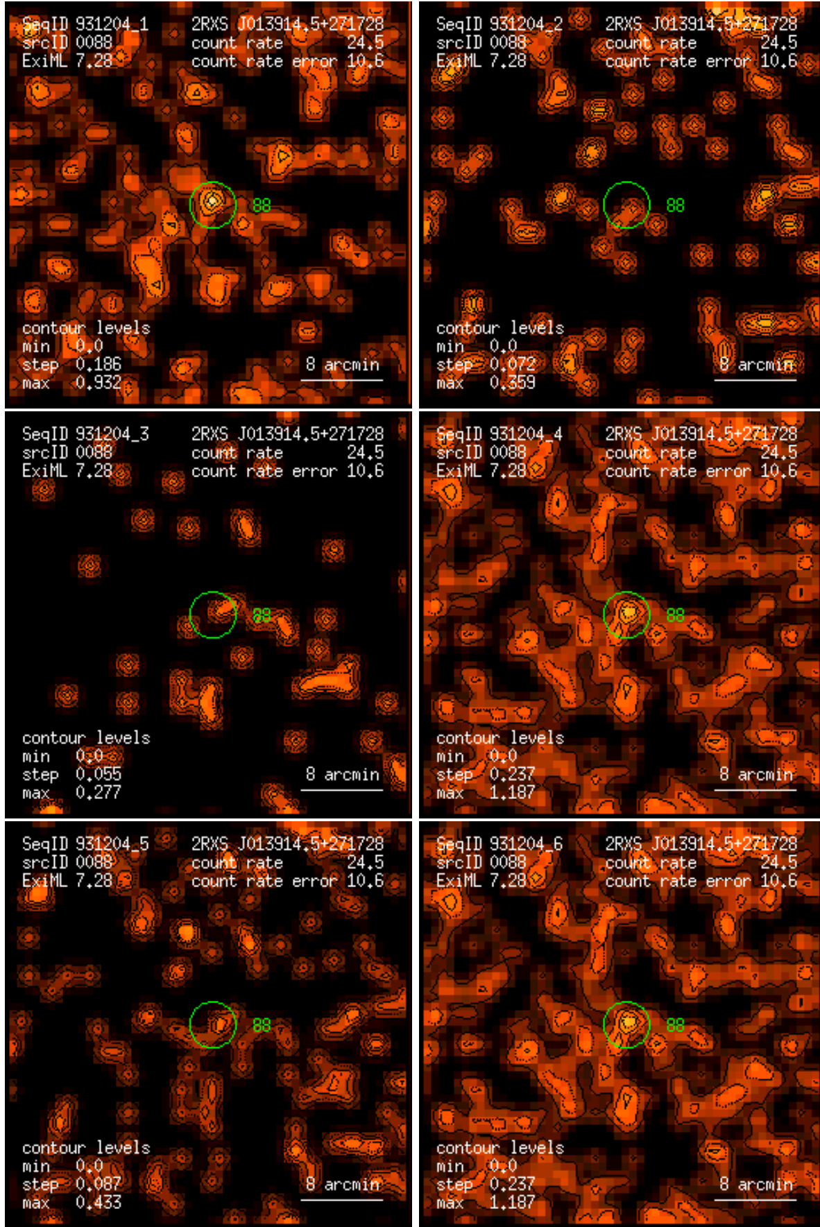
Figure 88: RASS 931204: detection 0088: band rate images, Gaussian filter: (1) PSPC channels 11 – 41, (2) 52 – 90, (3) 91 – 201, (4) 11 – 235, (5) 52 – 201, (6) 11 – 201. Broad band rates in counts/ks. Band rate contour levels in counts/ks/arcmin 2 .
