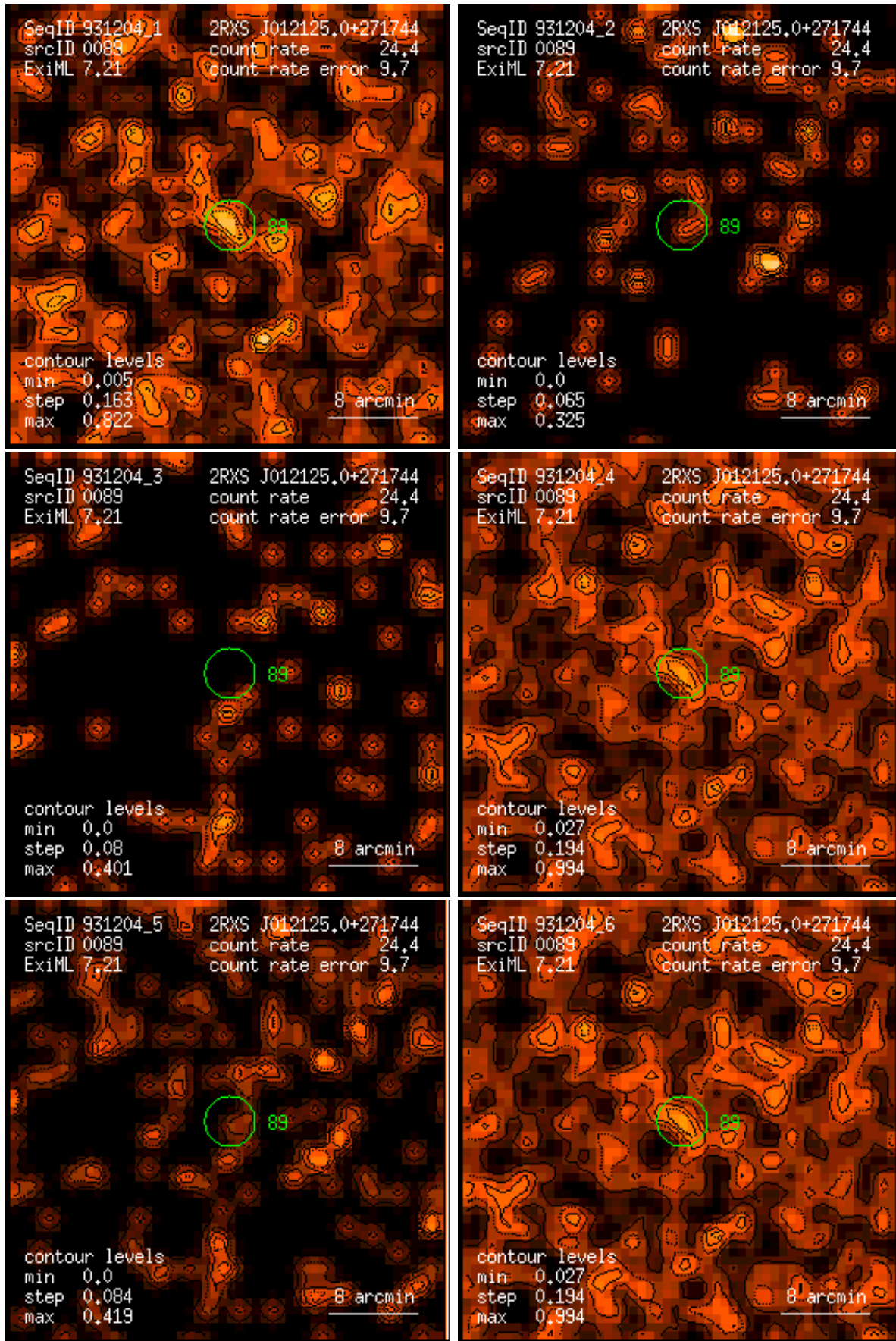
Figure 89: RASS 931204: detection 0089: band rate images, Gaussian filter: (1) PSPC channels 11 – 41, (2) 52 – 90, (3) 91 – 201, (4) 11 – 235, (5) 52 – 201, (6) 11 – 201. Broad band rates in counts/ks. Band rate contour levels in counts/ks/arcmin 2 .
