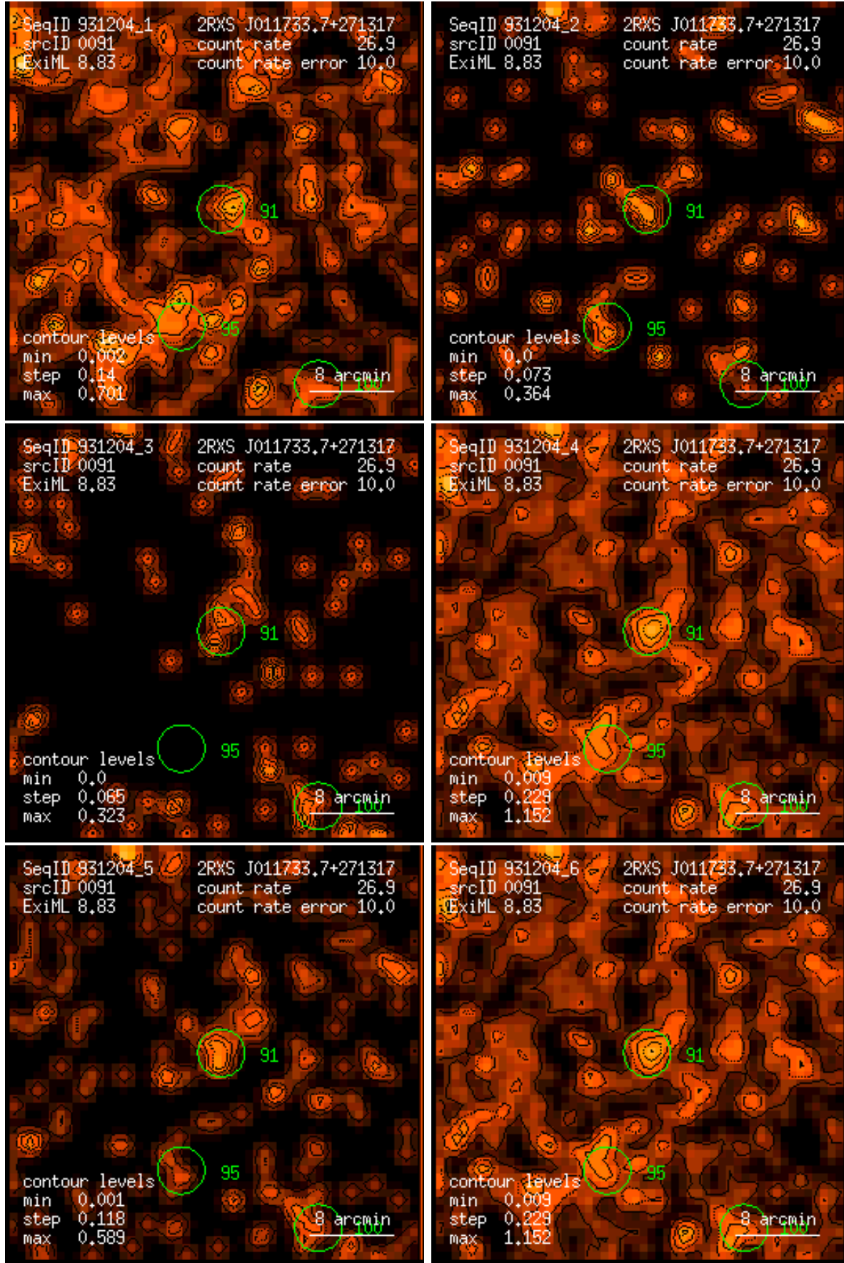
Figure 91: RASS 931204: detection 0091: band rate images, Gaussian filter: (1) PSPC channels 11 – 41, (2) 52 – 90, (3) 91 – 201, (4) 11 – 235, (5) 52 – 201, (6) 11 – 201. Broad band rates in counts/ks. Band rate contour levels in counts/ks/arcmin 2 .
