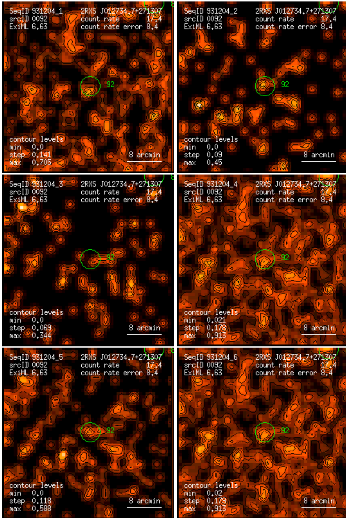
Figure 92: RASS 931204: detection 0092: band rate images, Gaussian filter: (1) PSPC channels 11 – 41, (2) 52 – 90, (3) 91 – 201, (4) 11 – 235, (5) 52 – 201, (6) 11 – 201. Broad band rates in counts/ks. Band rate contour levels in counts/ks/arcmin 2 .
