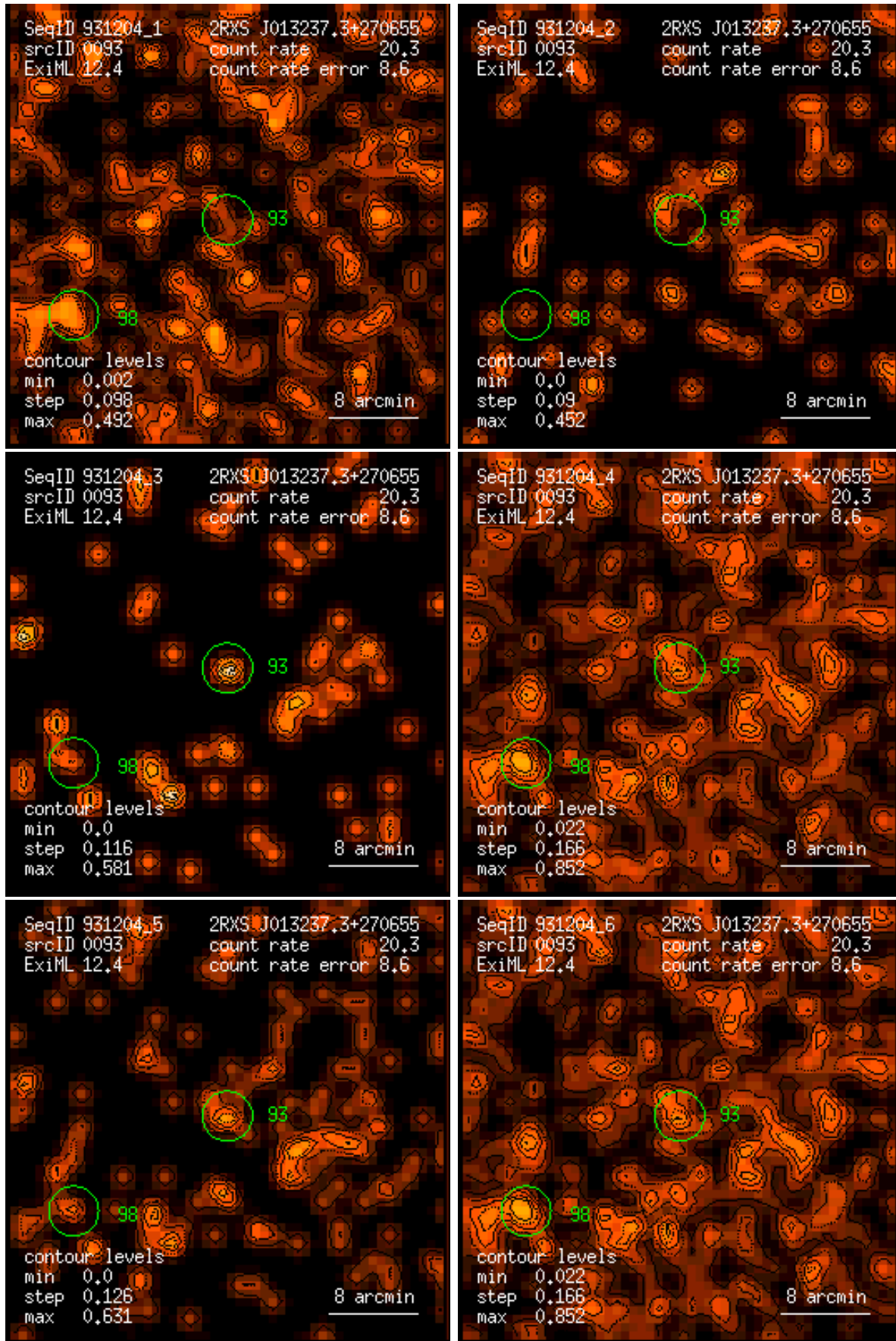
Figure 93: RASS 931204: detection 0093: band rate images, Gaussian filter: (1) PSPC channels 11 – 41, (2) 52 – 90, (3) 91 – 201, (4) 11 – 235, (5) 52 – 201, (6) 11 – 201. Broad band rates in counts/ks. Band rate contour levels in counts/ks/arcmin 2 .
