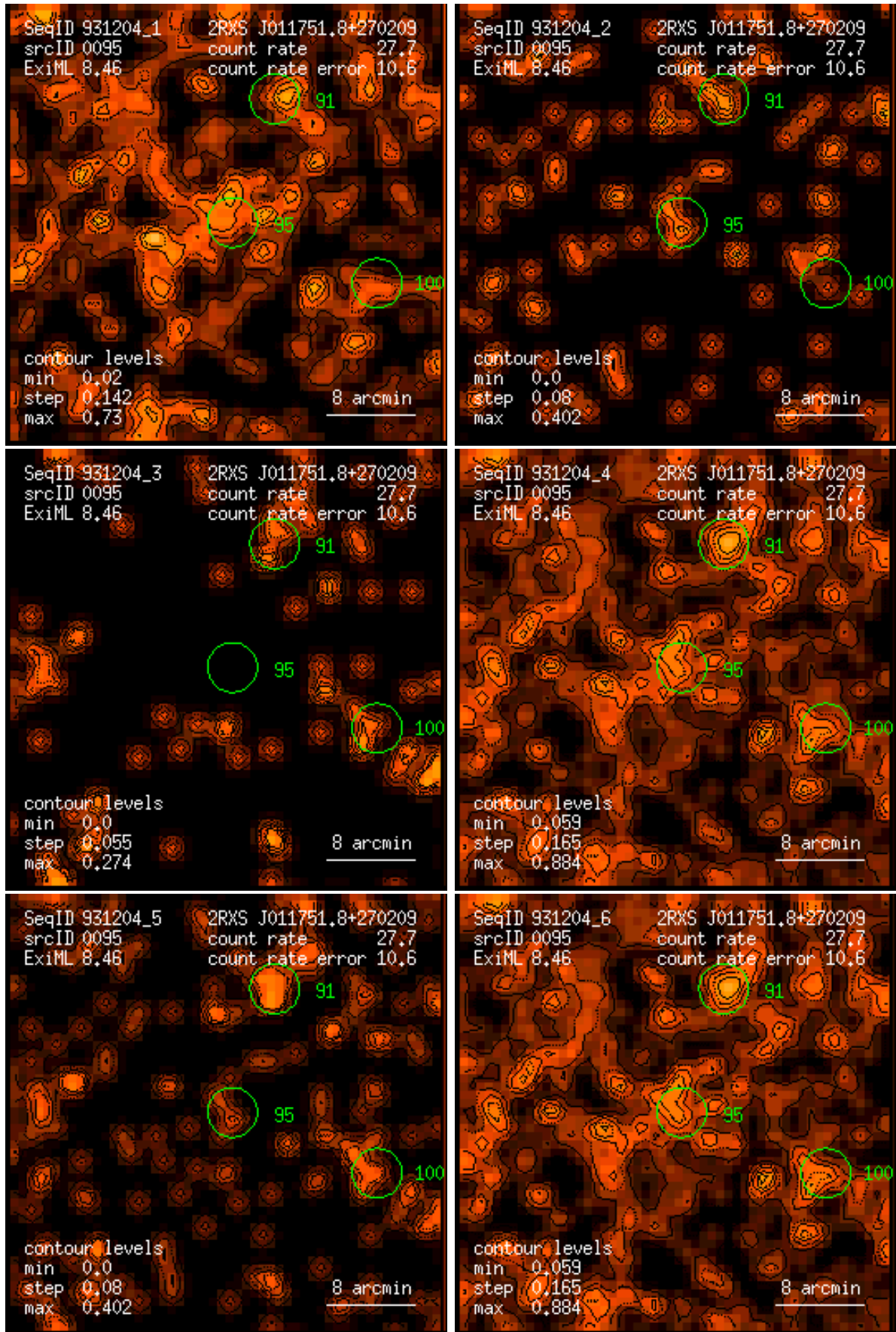
Figure 95: RASS 931204: detection 0095: band rate images, Gaussian filter: (1) PSPC channels 11 – 41, (2) 52 – 90, (3) 91 – 201, (4) 11 – 235, (5) 52 – 201, (6) 11 – 201. Broad band rates in counts/ks. Band rate contour levels in counts/ks/arcmin 2 .
