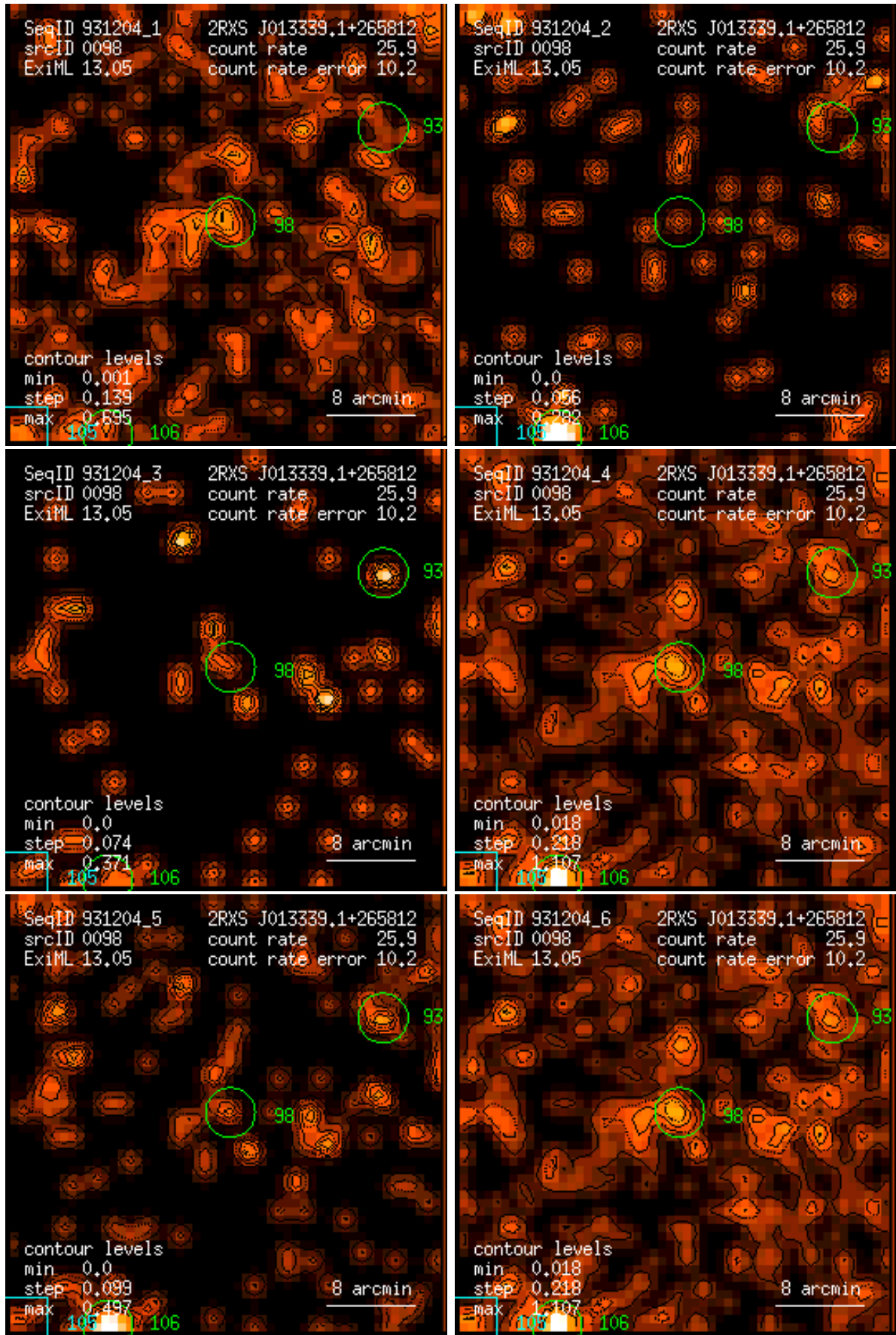
Figure 98: RASS 931204: detection 0098: band rate images, Gaussian filter: (1) PSPC channels 11 – 41, (2) 52 – 90, (3) 91 – 201, (4) 11 – 235, (5) 52 – 201, (6) 11 – 201. Broad band rates in counts/ks. Band rate contour levels in counts/ks/arcmin 2 .
