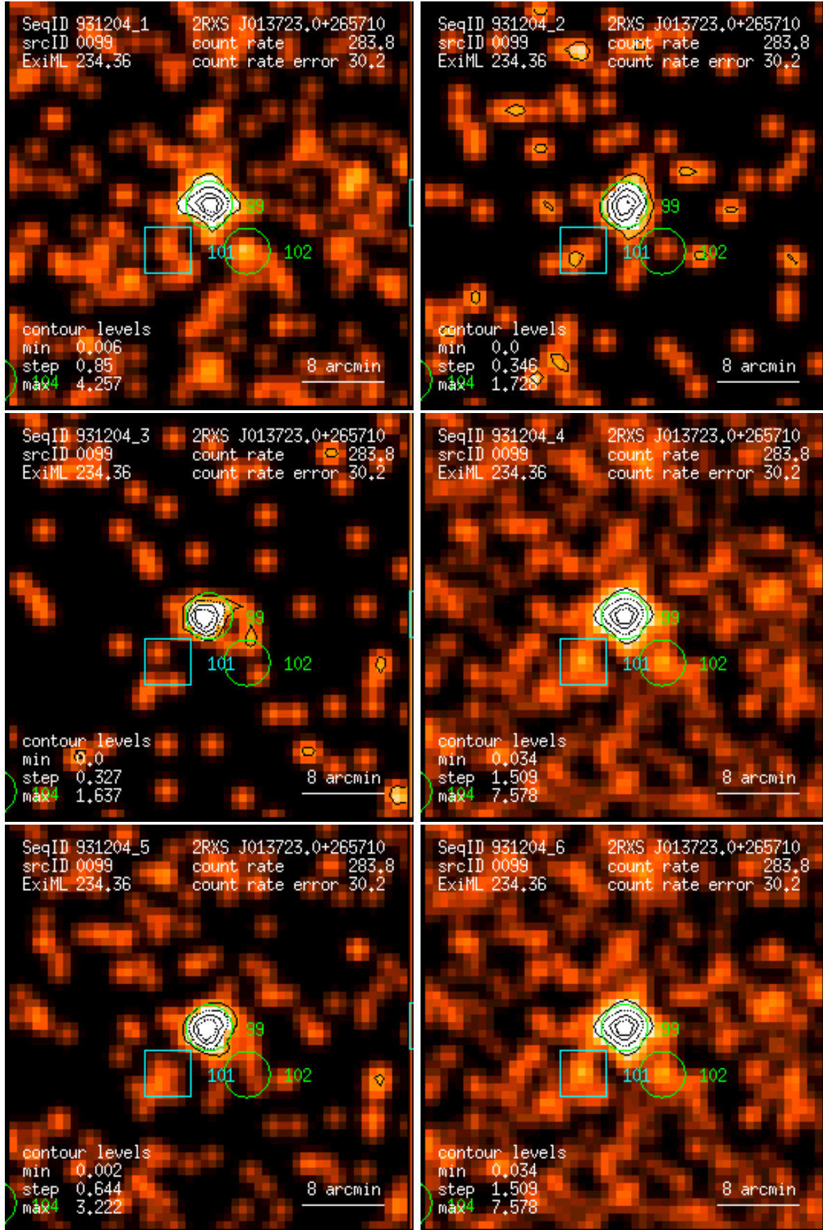
Figure 99: RASS 931204: detection 0099: band rate images, Gaussian filter: (1) PSPC channels 11 – 41, (2) 52 – 90, (3) 91 – 201, (4) 11 – 235, (5) 52 – 201, (6) 11 – 201. Broad band rates in counts/ks. Band rate contour levels in counts/ks/arcmin 2 .
