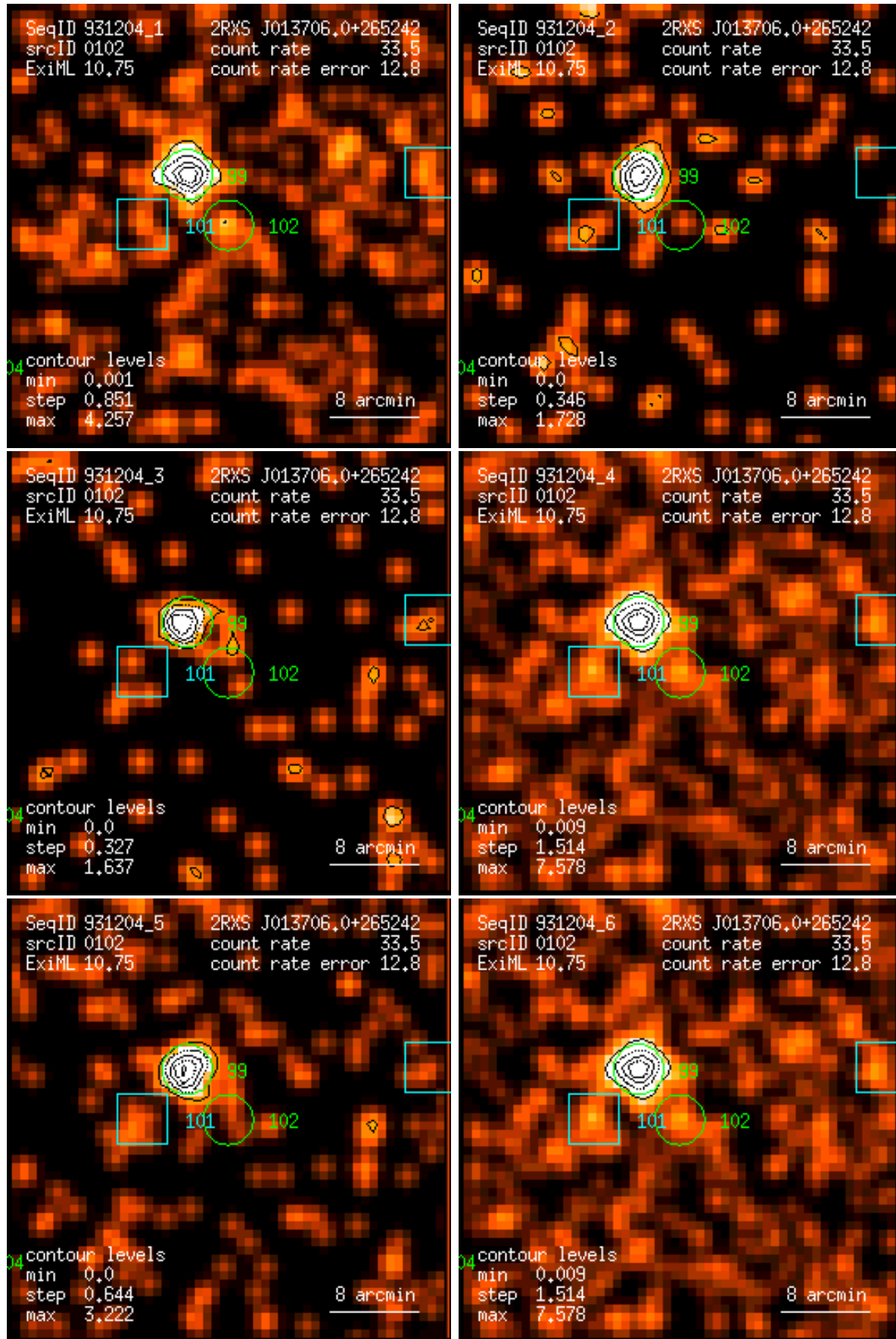
Figure 102: RASS 931204: detection 0102: band rate images, Gaussian filter: (1) PSPC channels 11 – 41, (2) 52 – 90, (3) 91 – 201, (4) 11 – 235, (5) 52 – 201, (6) 11 – 201. Broad band rates in counts/ks. Band rate contour levels in counts/ks/arcmin 2 .
