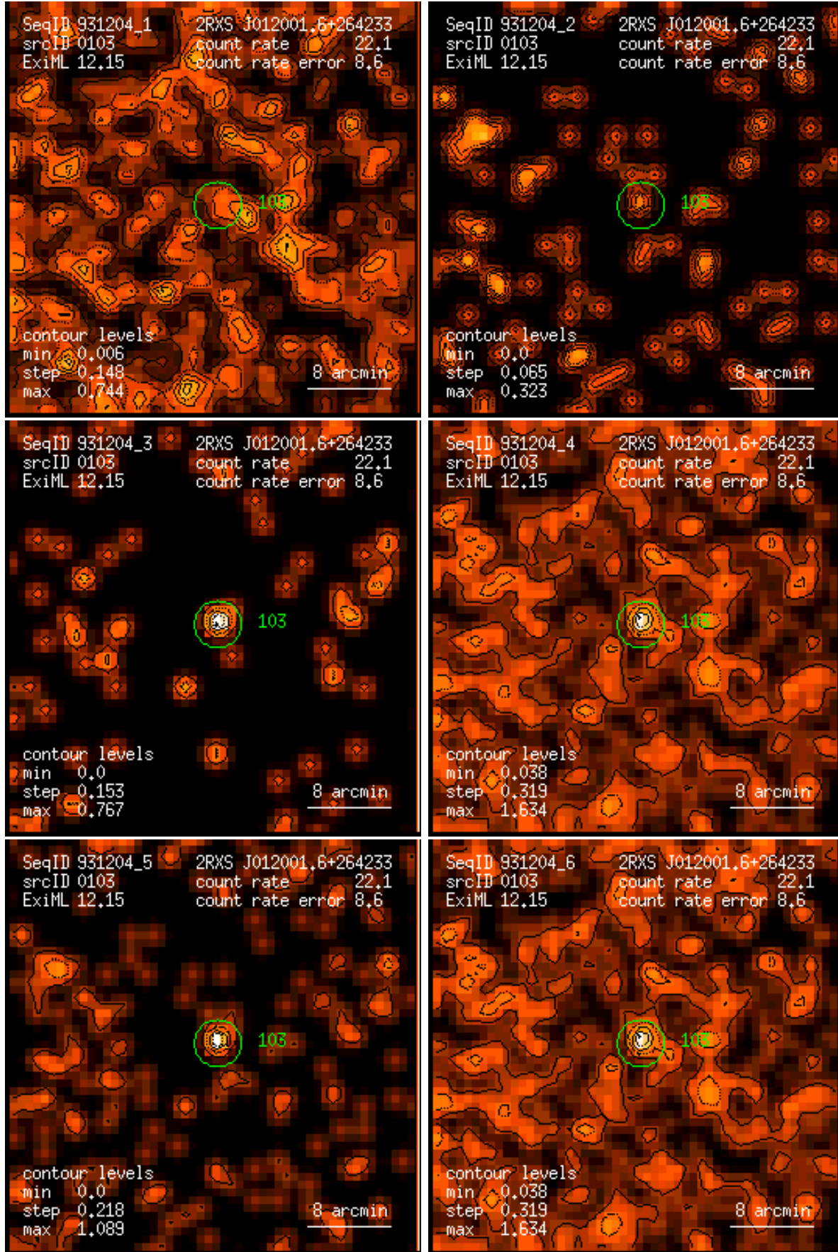
Figure 103: RASS 931204: detection 0103: band rate images, Gaussian filter: (1) PSPC channels 11 – 41, (2) 52 – 90, (3) 91 – 201, (4) 11 – 235, (5) 52 – 201, (6) 11 – 201. Broad band rates in counts/ks. Band rate contour levels in counts/ks/arcmin 2 .
