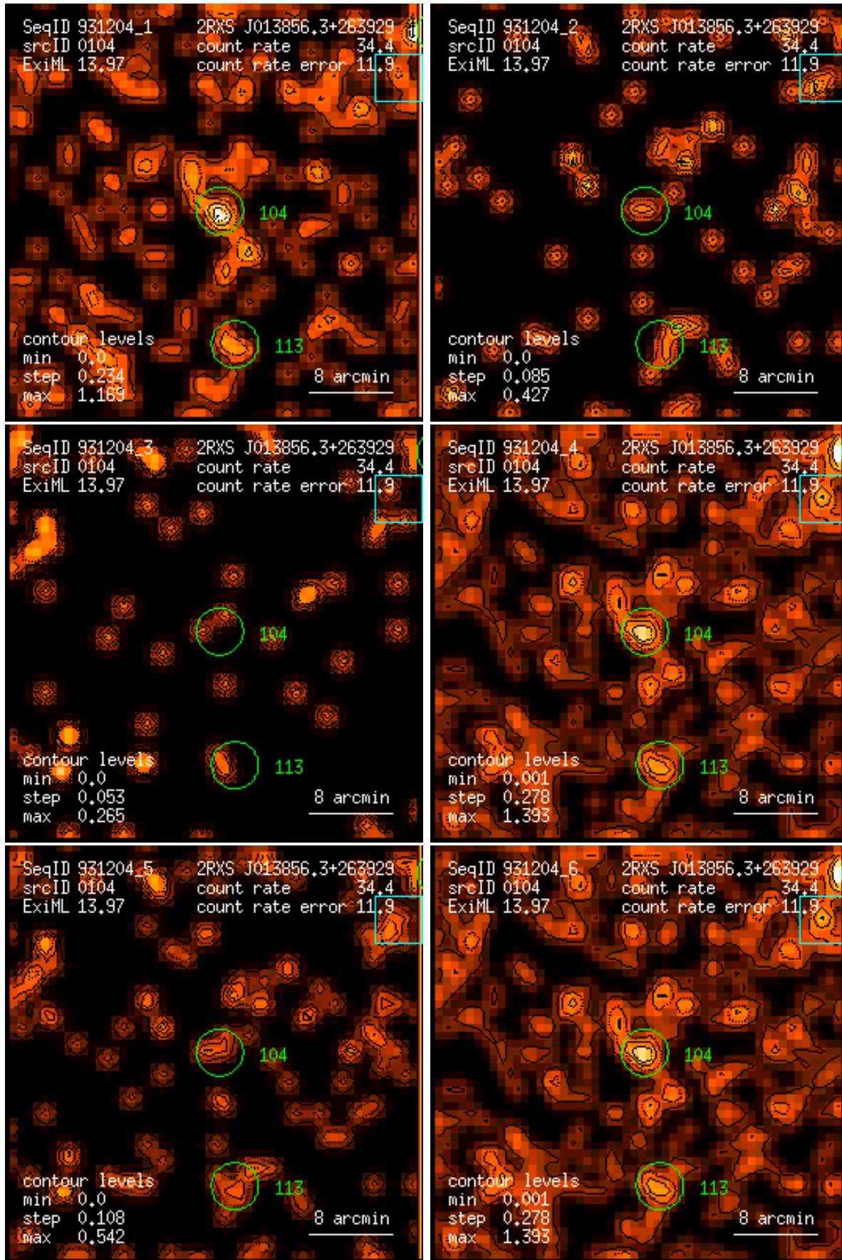
Figure 104: RASS 931204: detection 0104: band rate images, Gaussian filter: (1) PSPC channels 11 – 41, (2) 52 – 90, (3) 91 – 201, (4) 11 – 235, (5) 52 – 201, (6) 11 – 201. Broad band rates in counts/ks. Band rate contour levels in counts/ks/arcmin 2 .
