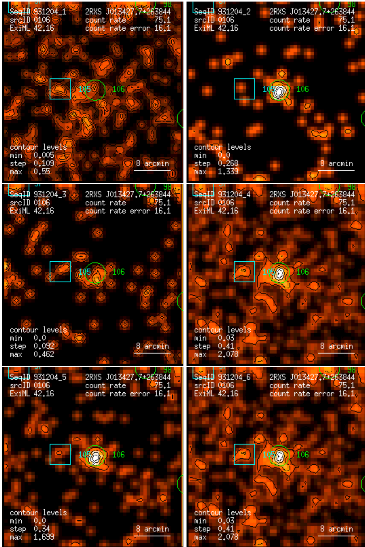
Figure 106: RASS 931204: detection 0106: band rate images, Gaussian filter: (1) PSPC channels 11 – 41, (2) 52 – 90, (3) 91 – 201, (4) 11 – 235, (5) 52 – 201, (6) 11 – 201. Broad band rates in counts/ks. Band rate contour levels in counts/ks/arcmin 2 .
