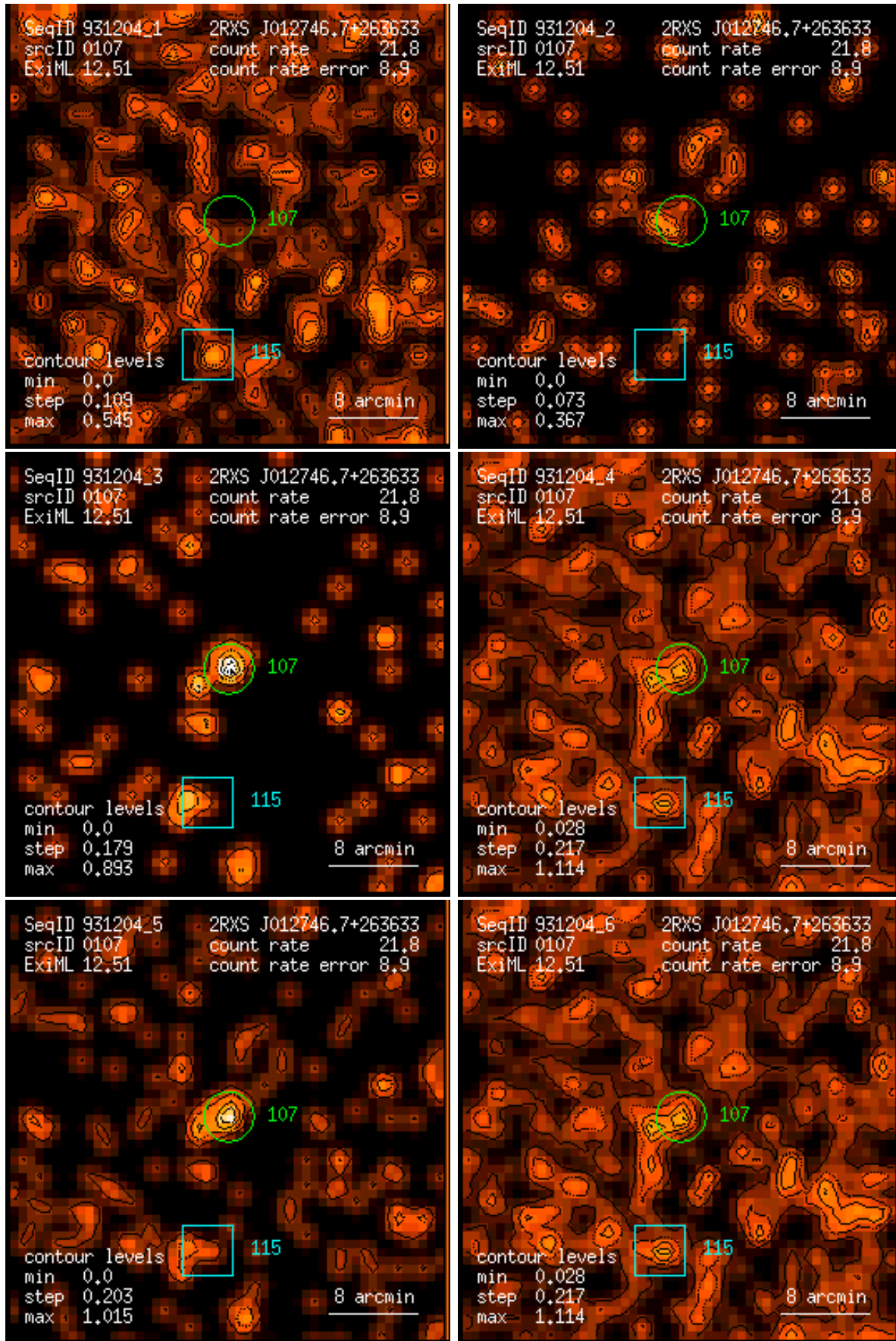
Figure 107: RASS 931204: detection 0107: band rate images, Gaussian filter: (1) PSPC channels 11 – 41, (2) 52 – 90, (3) 91 – 201, (4) 11 – 235, (5) 52 – 201, (6) 11 – 201. Broad band rates in counts/ks. Band rate contour levels in counts/ks/arcmin 2 .
