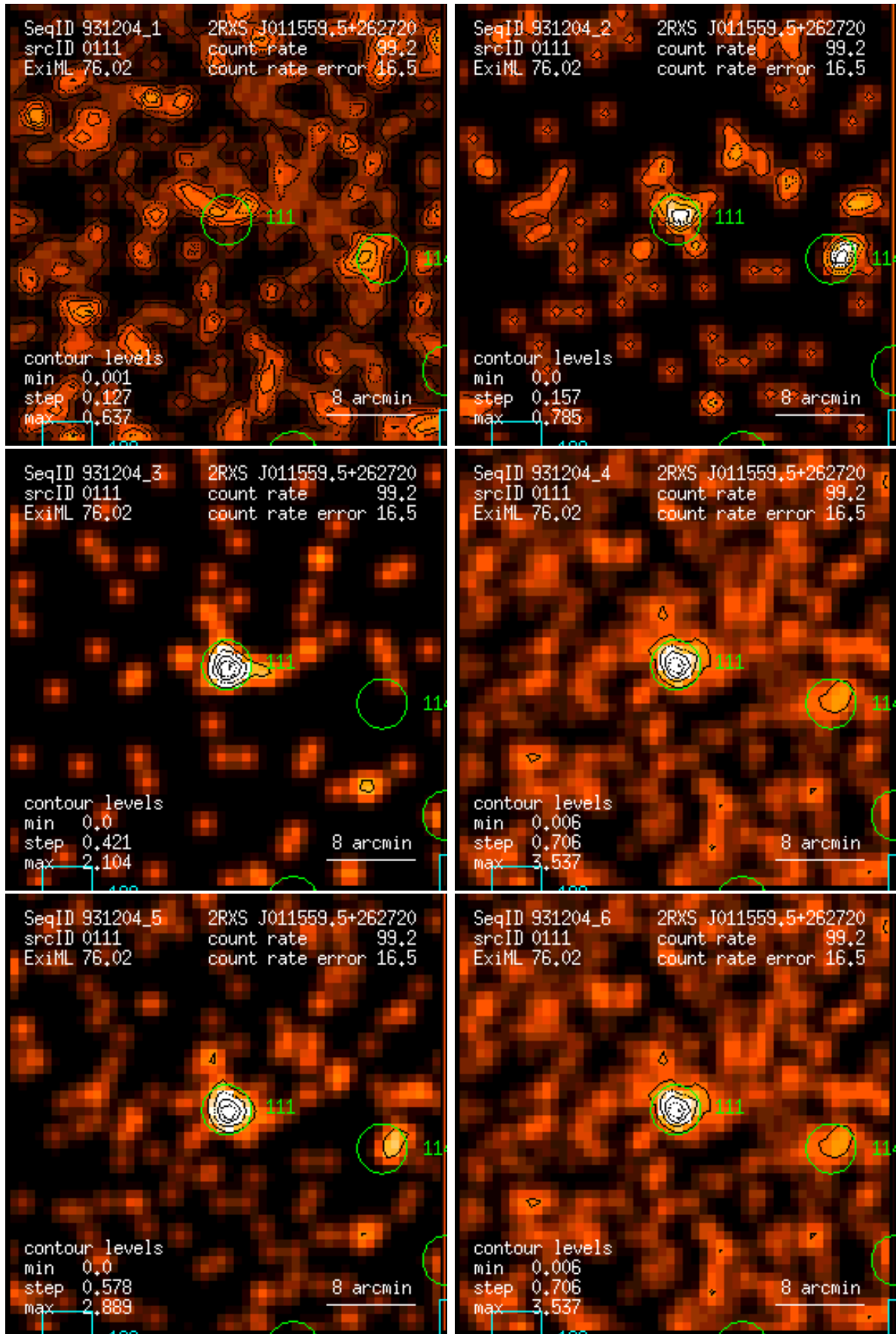
Figure 111: RASS 931204: detection 0111: band rate images, Gaussian filter: (1) PSPC channels 11 – 41, (2) 52 – 90, (3) 91 – 201, (4) 11 – 235, (5) 52 – 201, (6) 11 – 201. Broad band rates in counts/ks. Band rate contour levels in counts/ks/arcmin 2 .
