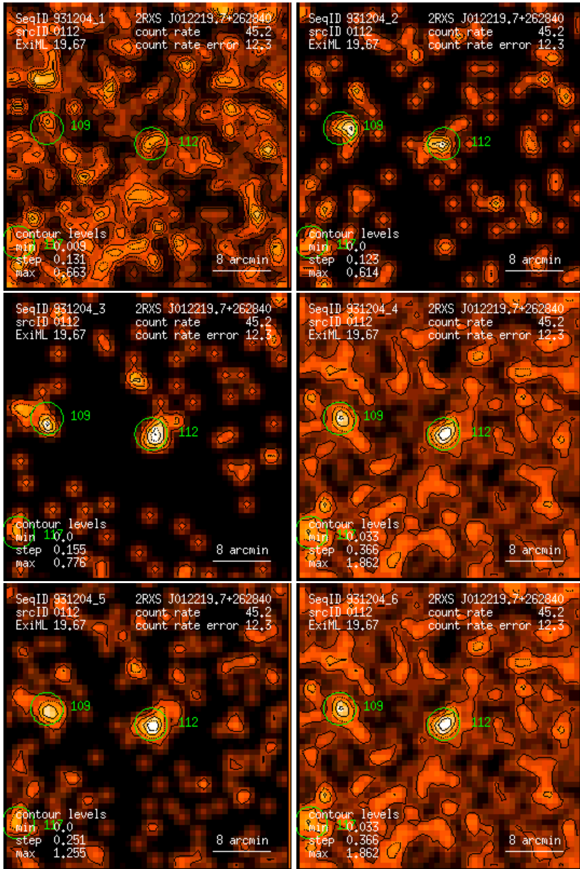
Figure 112: RASS 931204: detection 0112: band rate images, Gaussian filter: (1) PSPC channels 11 – 41, (2) 52 – 90, (3) 91 – 201, (4) 11 – 235, (5) 52 – 201, (6) 11 – 201. Broad band rates in counts/ks. Band rate contour levels in counts/ks/arcmin 2 .
