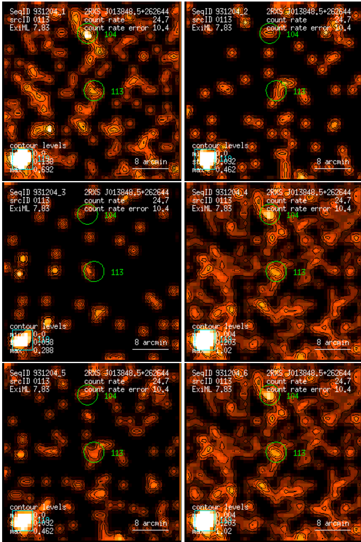
Figure 113: RASS 931204: detection 0113: band rate images, Gaussian filter: (1) PSPC channels 11 – 41, (2) 52 – 90, (3) 91 – 201, (4) 11 – 235, (5) 52 – 201, (6) 11 – 201. Broad band rates in counts/ks. Band rate contour levels in counts/ks/arcmin 2 .
