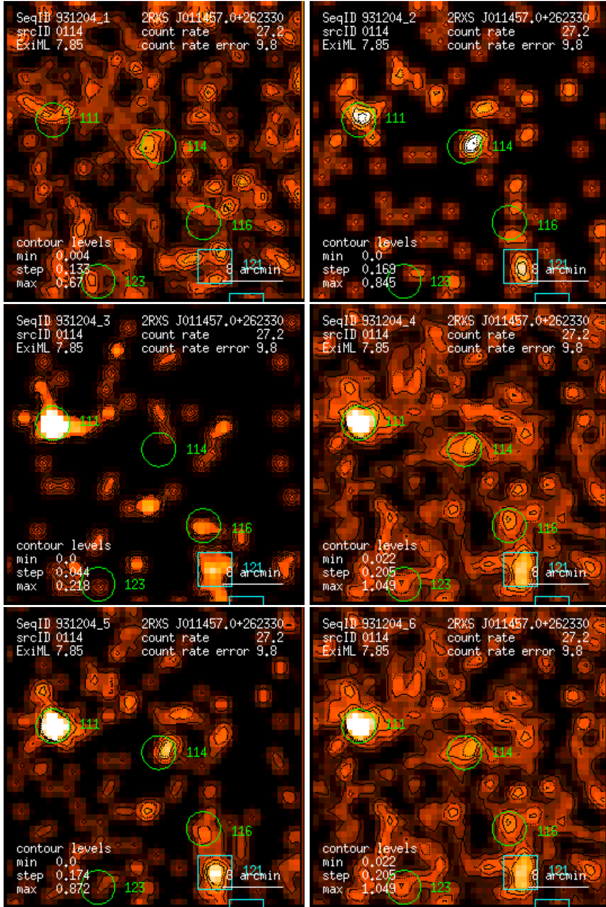
Figure 114: RASS 931204: detection 0114: band rate images, Gaussian filter: (1) PSPC channels 11 – 41, (2) 52 – 90, (3) 91 – 201, (4) 11 – 235, (5) 52 – 201, (6) 11 – 201. Broad band rates in counts/ks. Band rate contour levels in counts/ks/arcmin 2 .
