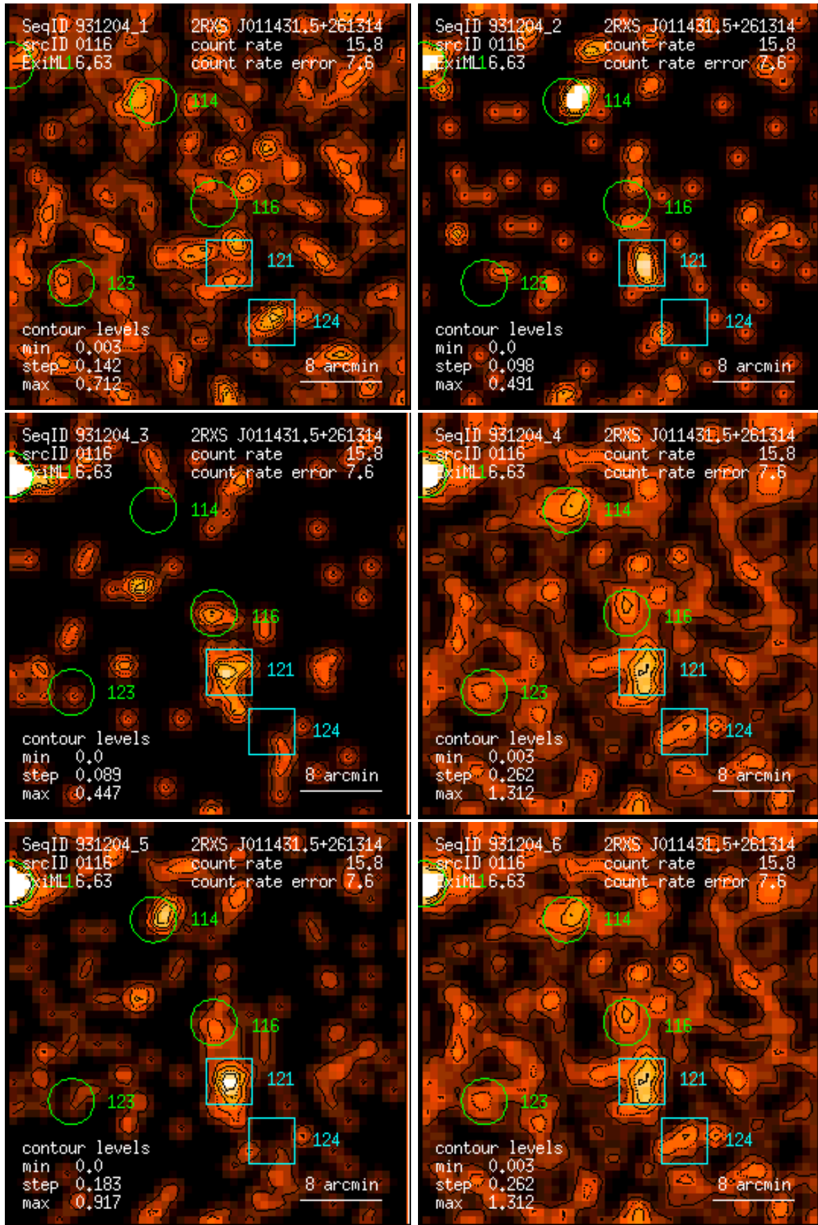
Figure 116: RASS 931204: detection 0116: band rate images, Gaussian filter: (1) PSPC channels 11 – 41, (2) 52 – 90, (3) 91 – 201, (4) 11 – 235, (5) 52 – 201, (6) 11 – 201. Broad band rates in counts/ks. Band rate contour levels in counts/ks/arcmin 2 .
