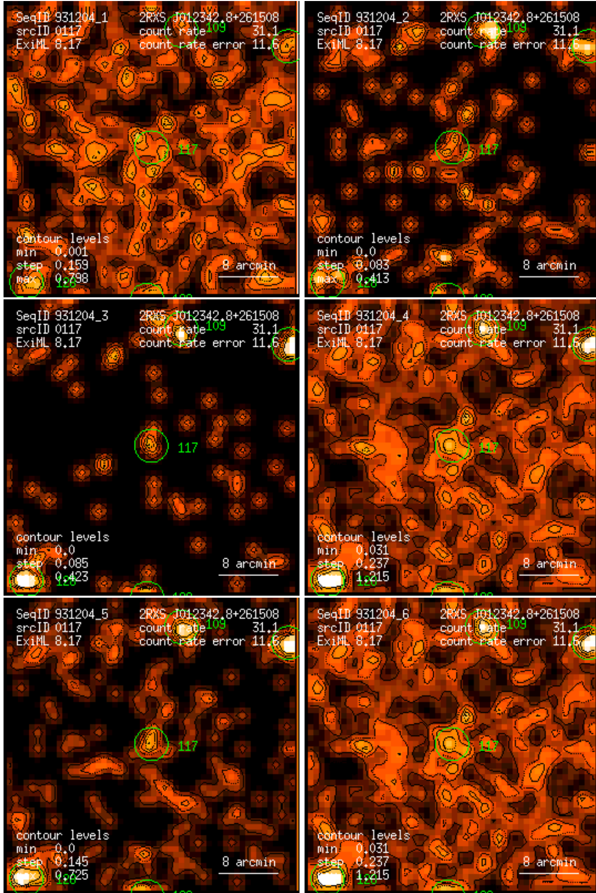
Figure 117: RASS 931204: detection 0117: band rate images, Gaussian filter: (1) PSPC channels 11 – 41, (2) 52 – 90, (3) 91 – 201, (4) 11 – 235, (5) 52 – 201, (6) 11 – 201. Broad band rates in counts/ks. Band rate contour levels in counts/ks/arcmin 2 .
