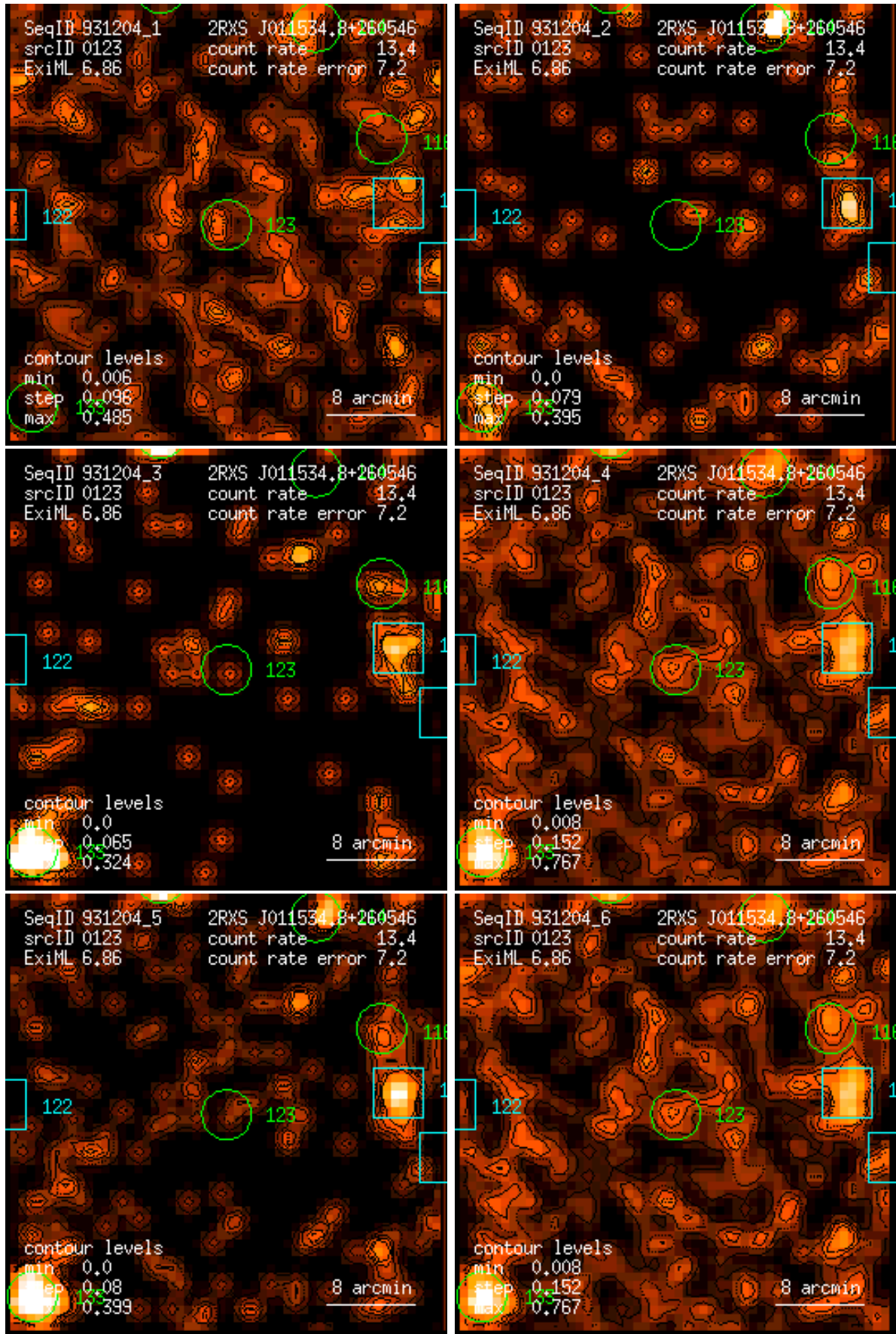
Figure 123: RASS 931204: detection 0123: band rate images, Gaussian filter: (1) PSPC channels 11 – 41, (2) 52 – 90, (3) 91 – 201, (4) 11 – 235, (5) 52 – 201, (6) 11 – 201. Broad band rates in counts/ks. Band rate contour levels in counts/ks/arcmin 2 .
