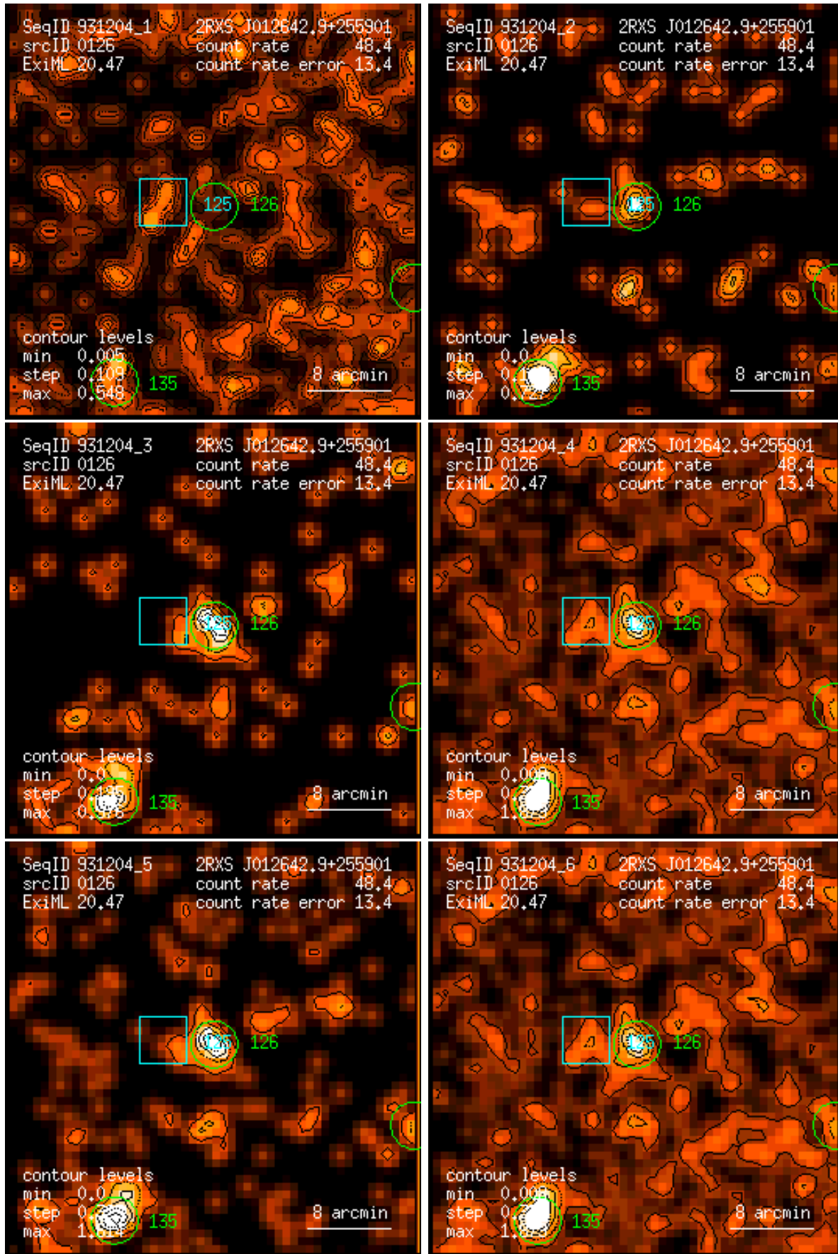
Figure 126: RASS 931204: detection 0126: band rate images, Gaussian filter: (1) PSPC channels 11 – 41, (2) 52 – 90, (3) 91 – 201, (4) 11 – 235, (5) 52 – 201, (6) 11 – 201. Broad band rates in counts/ks. Band rate contour levels in counts/ks/arcmin 2 .
