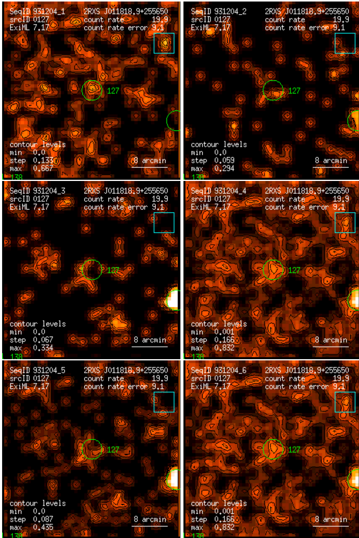
Figure 127: RASS 931204: detection 0127: band rate images, Gaussian filter: (1) PSPC channels 11 – 41, (2) 52 – 90, (3) 91 – 201, (4) 11 – 235, (5) 52 – 201, (6) 11 – 201. Broad band rates in counts/ks. Band rate contour levels in counts/ks/arcmin 2 .
