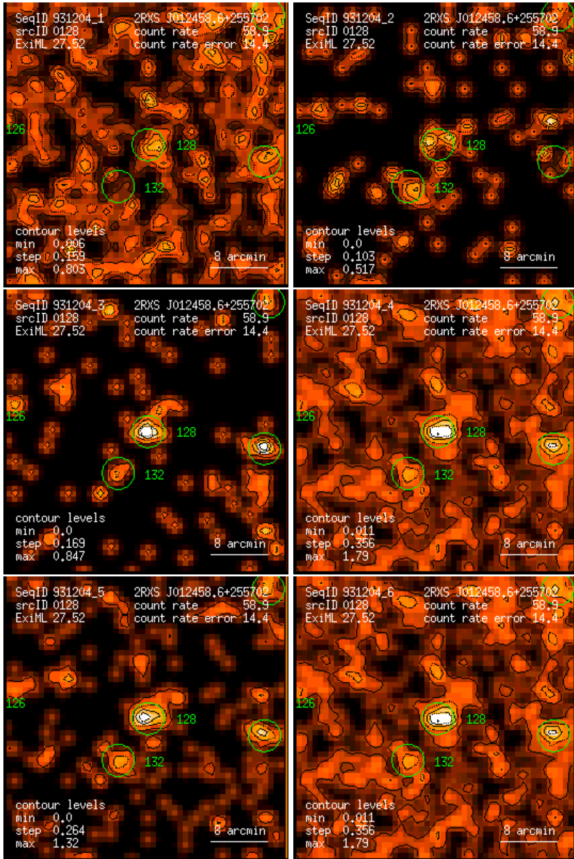
Figure 128: RASS 931204: detection 0128: band rate images, Gaussian filter: (1) PSPC channels 11 – 41, (2) 52 – 90, (3) 91 – 201, (4) 11 – 235, (5) 52 – 201, (6) 11 – 201. Broad band rates in counts/ks. Band rate contour levels in counts/ks/arcmin 2 .
