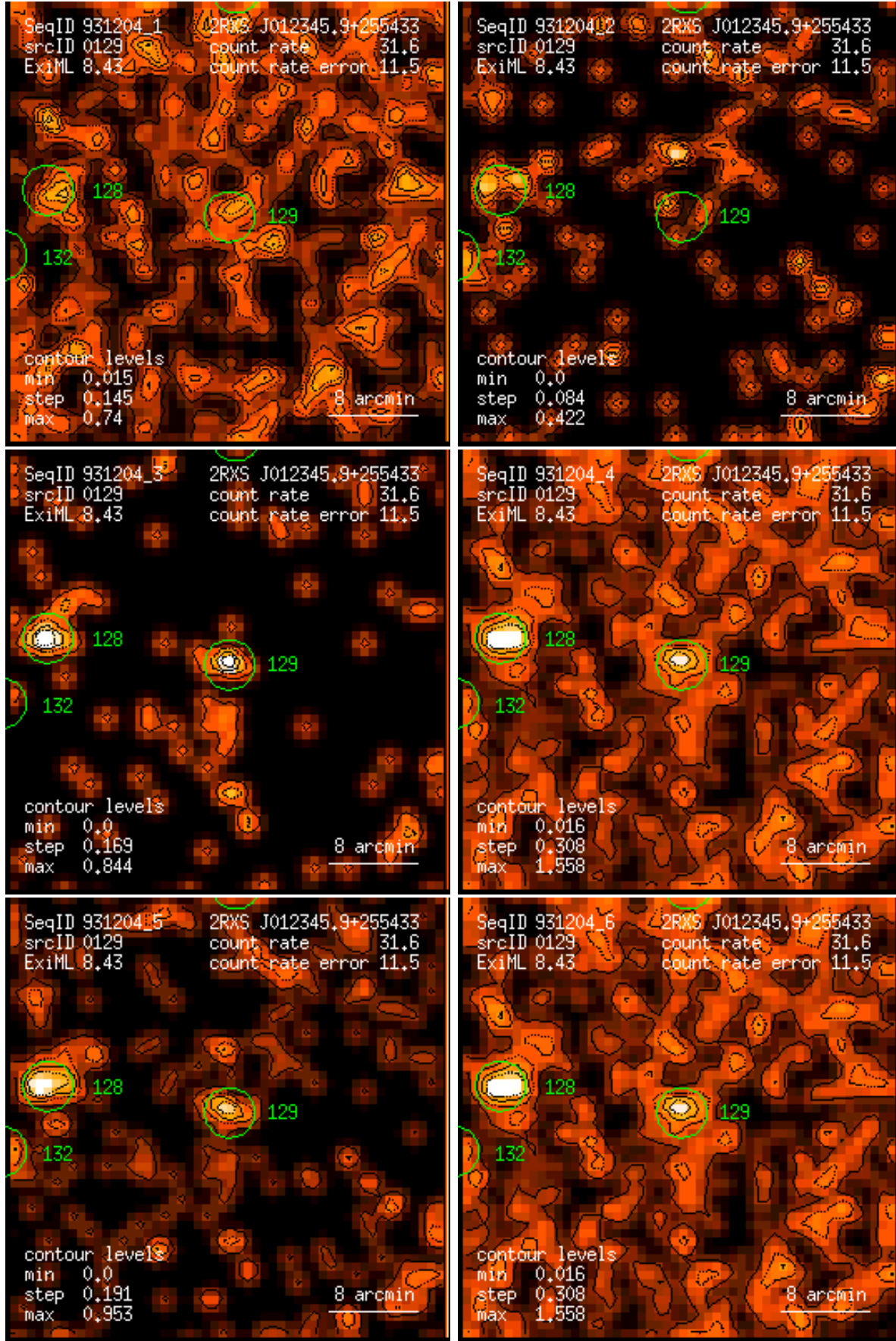
Figure 129: RASS 931204: detection 0129: band rate images, Gaussian filter: (1) PSPC channels 11 – 41, (2) 52 – 90, (3) 91 – 201, (4) 11 – 235, (5) 52 – 201, (6) 11 – 201. Broad band rates in counts/ks. Band rate contour levels in counts/ks/arcmin 2 .
