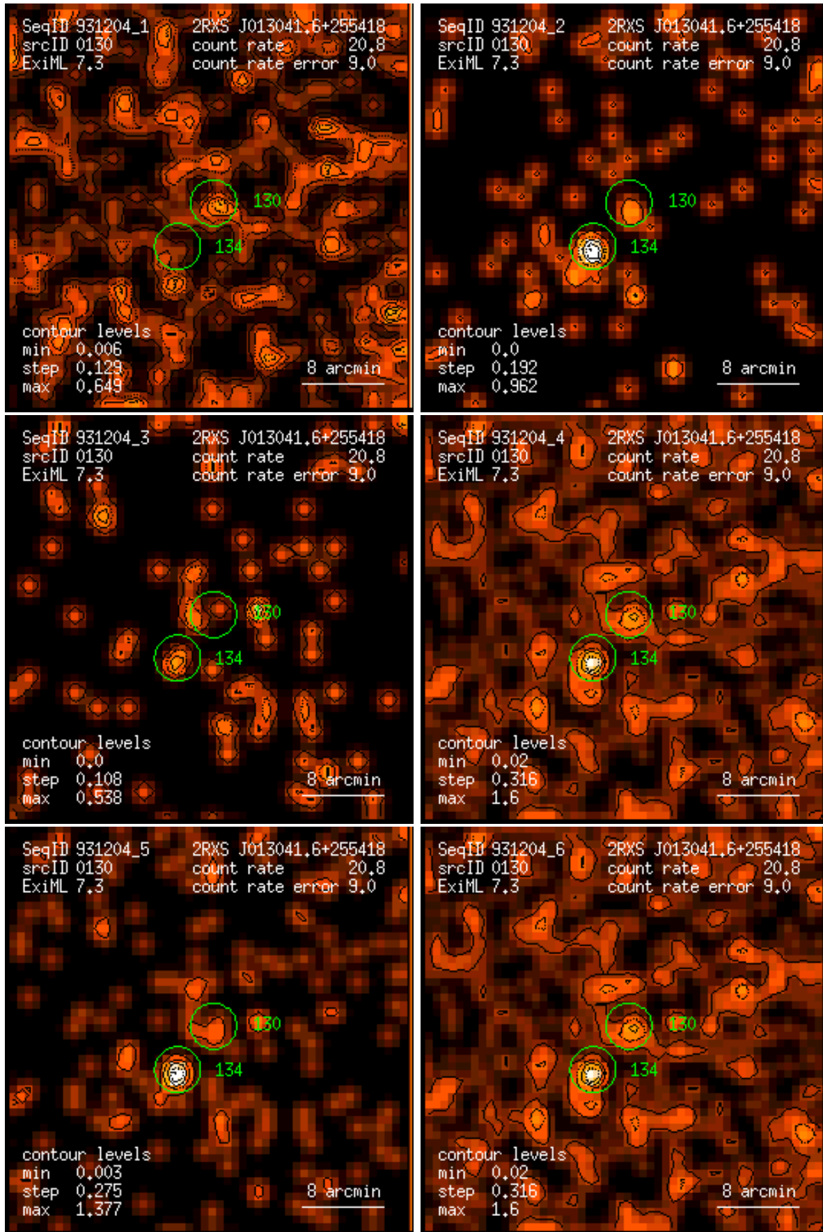
Figure 130: RASS 931204: detection 0130: band rate images, Gaussian filter: (1) PSPC channels 11 – 41, (2) 52 – 90, (3) 91 – 201, (4) 11 – 235, (5) 52 – 201, (6) 11 – 201. Broad band rates in counts/ks. Band rate contour levels in counts/ks/arcmin 2 .
