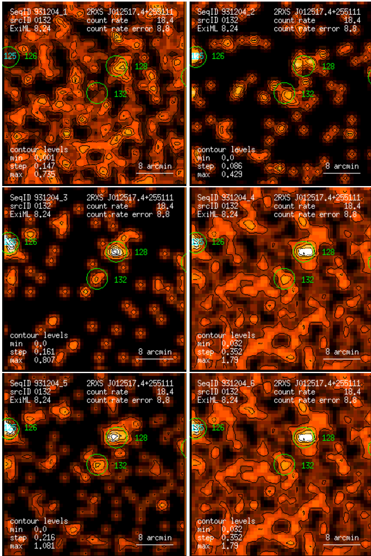
Figure 132: RASS 931204: detection 0132: band rate images, Gaussian filter: (1) PSPC channels 11 – 41, (2) 52 – 90, (3) 91 – 201, (4) 11 – 235, (5) 52 – 201, (6) 11 – 201. Broad band rates in counts/ks. Band rate contour levels in counts/ks/arcmin 2 .
