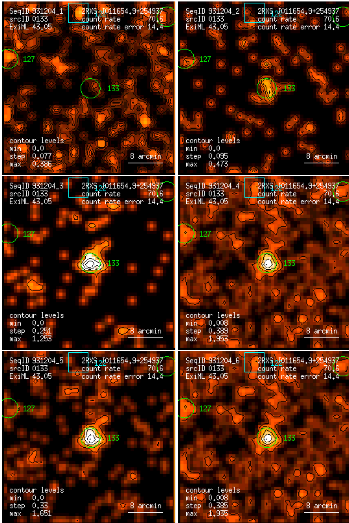
Figure 133: RASS 931204: detection 0133: band rate images, Gaussian filter: (1) PSPC channels 11 – 41, (2) 52 – 90, (3) 91 – 201, (4) 11 – 235, (5) 52 – 201, (6) 11 – 201. Broad band rates in counts/ks. Band rate contour levels in counts/ks/arcmin 2 .
