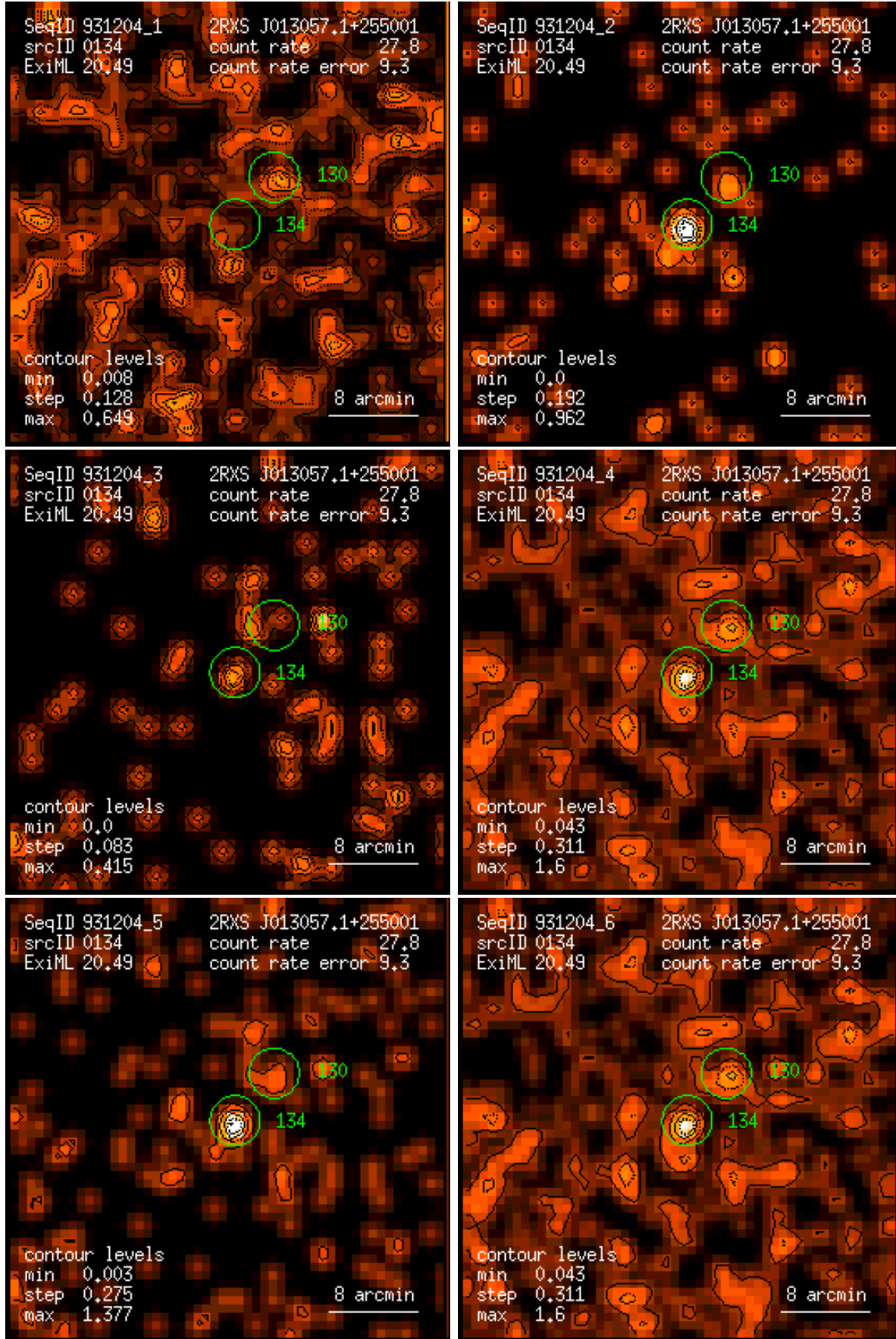
Figure 134: RASS 931204: detection 0134: band rate images, Gaussian filter: (1) PSPC channels 11 – 41, (2) 52 – 90, (3) 91 – 201, (4) 11 – 235, (5) 52 – 201, (6) 11 – 201. Broad band rates in counts/ks. Band rate contour levels in counts/ks/arcmin 2 .
