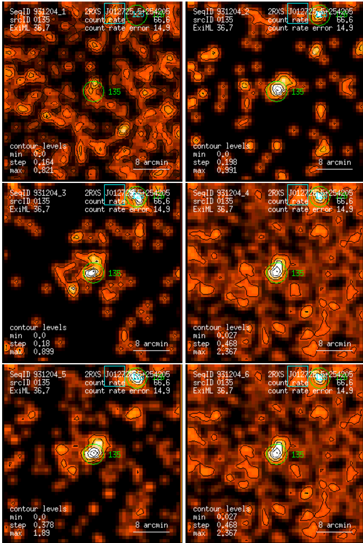
Figure 135: RASS 931204: detection 0135: band rate images, Gaussian filter: (1) PSPC channels 11 – 41, (2) 52 – 90, (3) 91 – 201, (4) 11 – 235, (5) 52 – 201, (6) 11 – 201. Broad band rates in counts/ks. Band rate contour levels in counts/ks/arcmin 2 .
