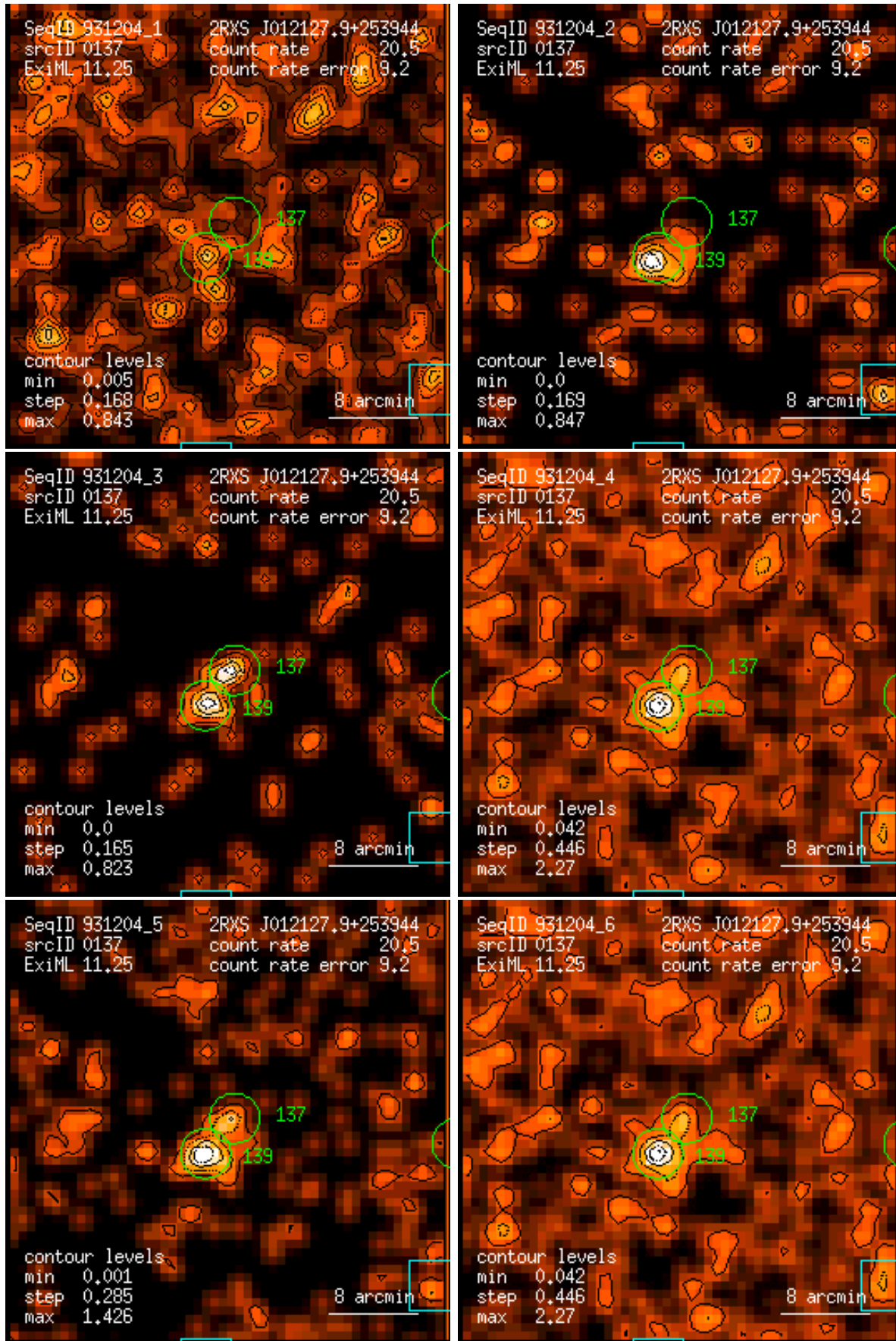
Figure 137: RASS 931204: detection 0137: band rate images, Gaussian filter: (1) PSPC channels 11 – 41, (2) 52 – 90, (3) 91 – 201, (4) 11 – 235, (5) 52 – 201, (6) 11 – 201. Broad band rates in counts/ks. Band rate contour levels in counts/ks/arcmin 2 .
