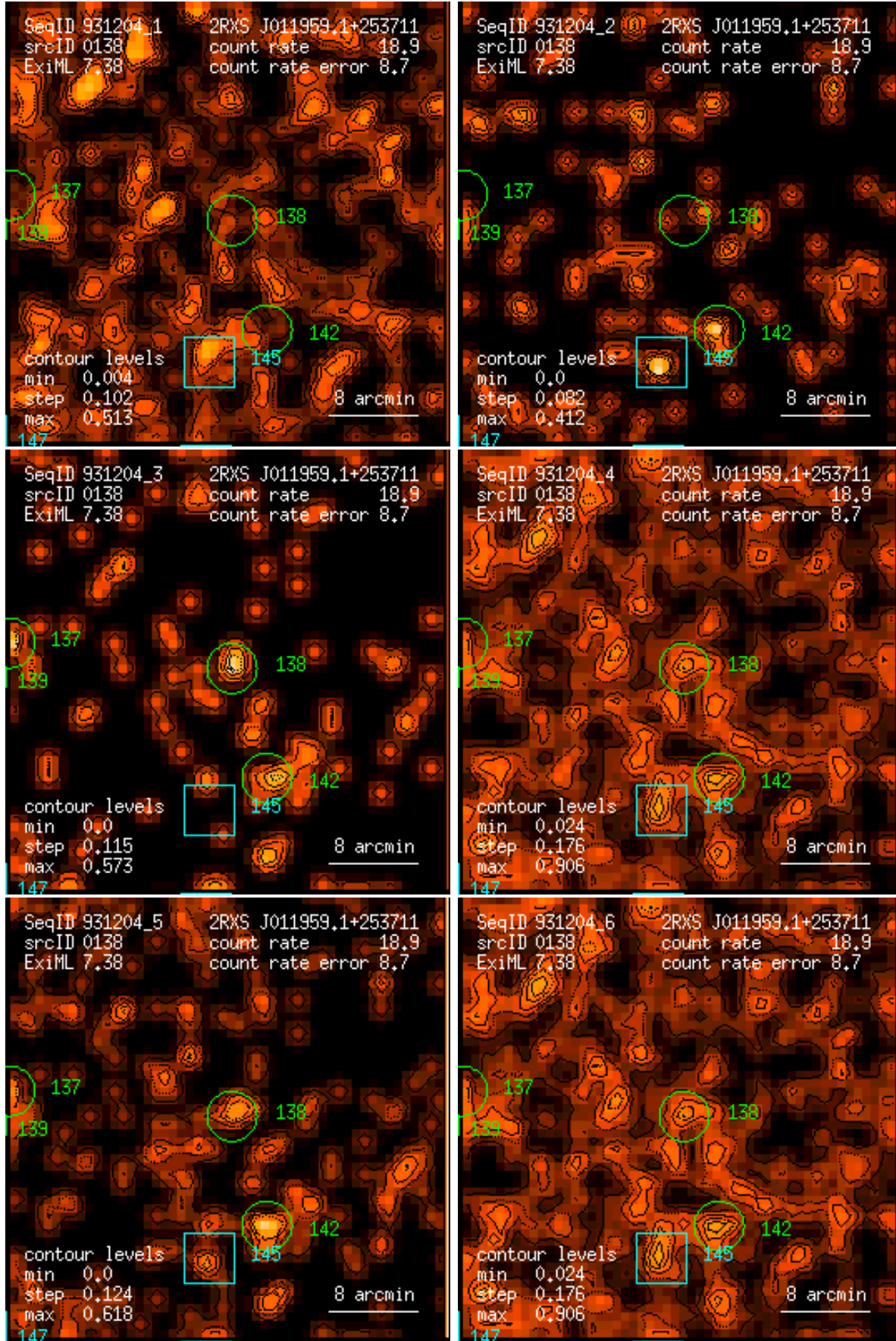
Figure 138: RASS 931204: detection 0138: band rate images, Gaussian filter: (1) PSPC channels 11 – 41, (2) 52 – 90, (3) 91 – 201, (4) 11 – 235, (5) 52 – 201, (6) 11 – 201. Broad band rates in counts/ks. Band rate contour levels in counts/ks/arcmin 2 .
