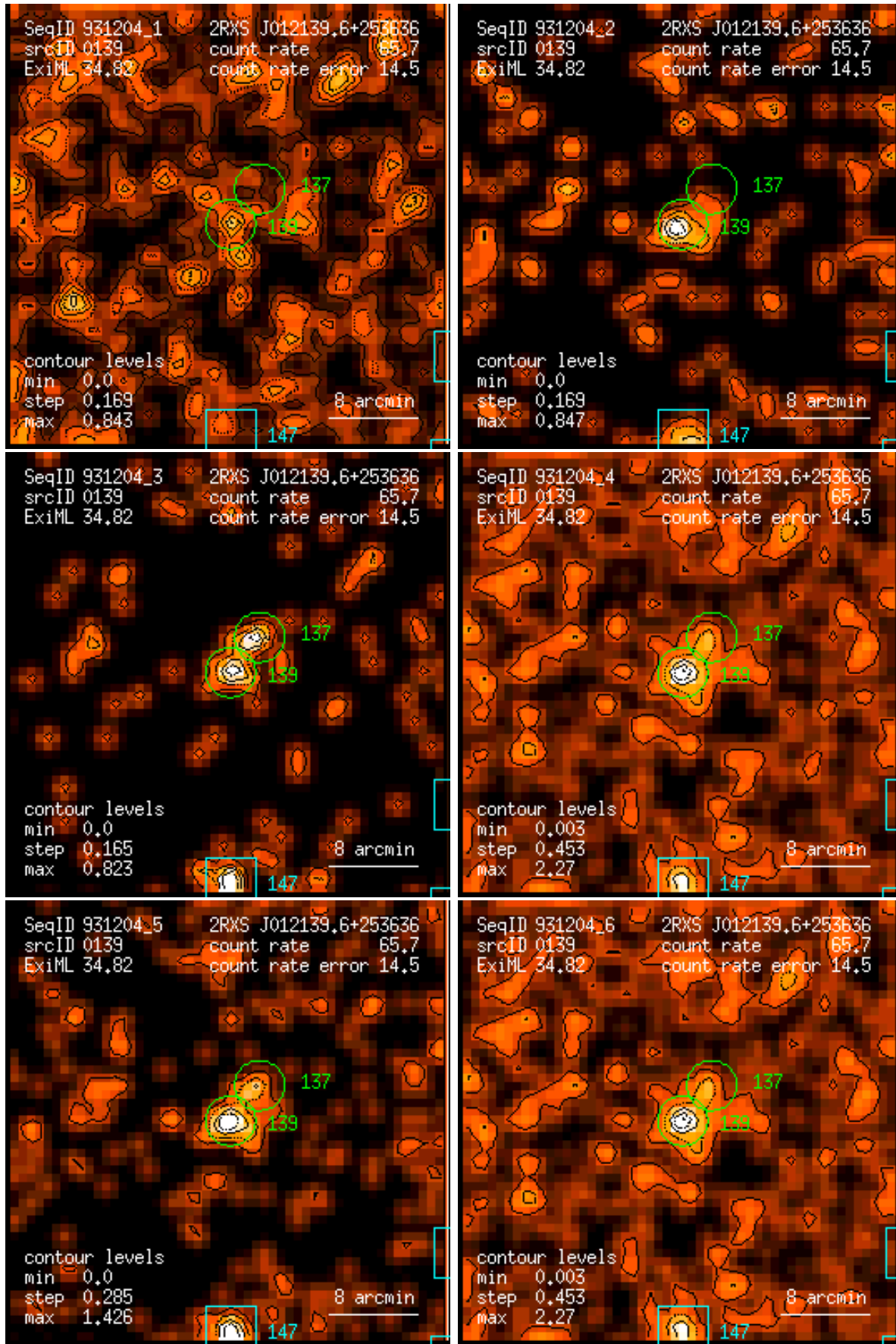
Figure 139: RASS 931204: detection 0139: band rate images, Gaussian filter: (1) PSPC channels 11 – 41, (2) 52 – 90, (3) 91 – 201, (4) 11 – 235, (5) 52 – 201, (6) 11 – 201. Broad band rates in counts/ks. Band rate contour levels in counts/ks/arcmin 2 .
