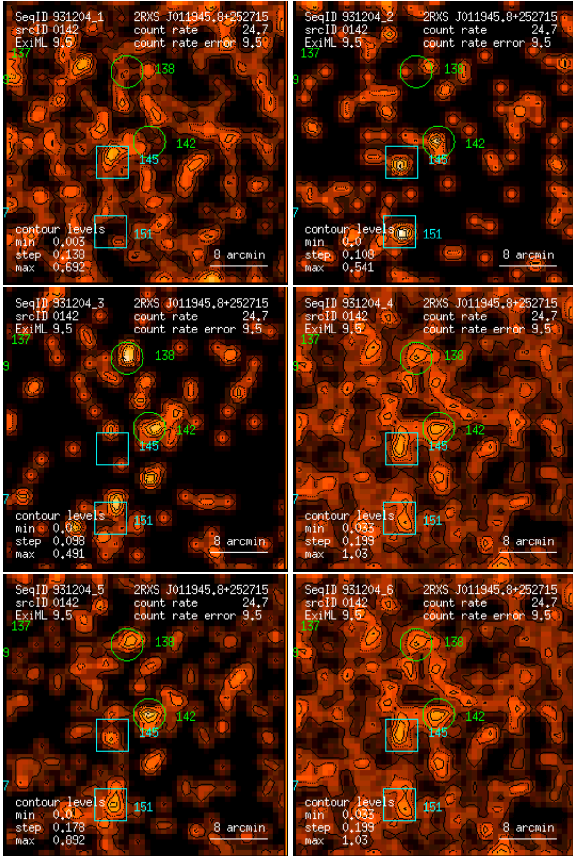
Figure 142: RASS 931204: detection 0142: band rate images, Gaussian filter: (1) PSPC channels 11 – 41, (2) 52 – 90, (3) 91 – 201, (4) 11 – 235, (5) 52 – 201, (6) 11 – 201. Broad band rates in counts/ks. Band rate contour levels in counts/ks/arcmin 2 .
