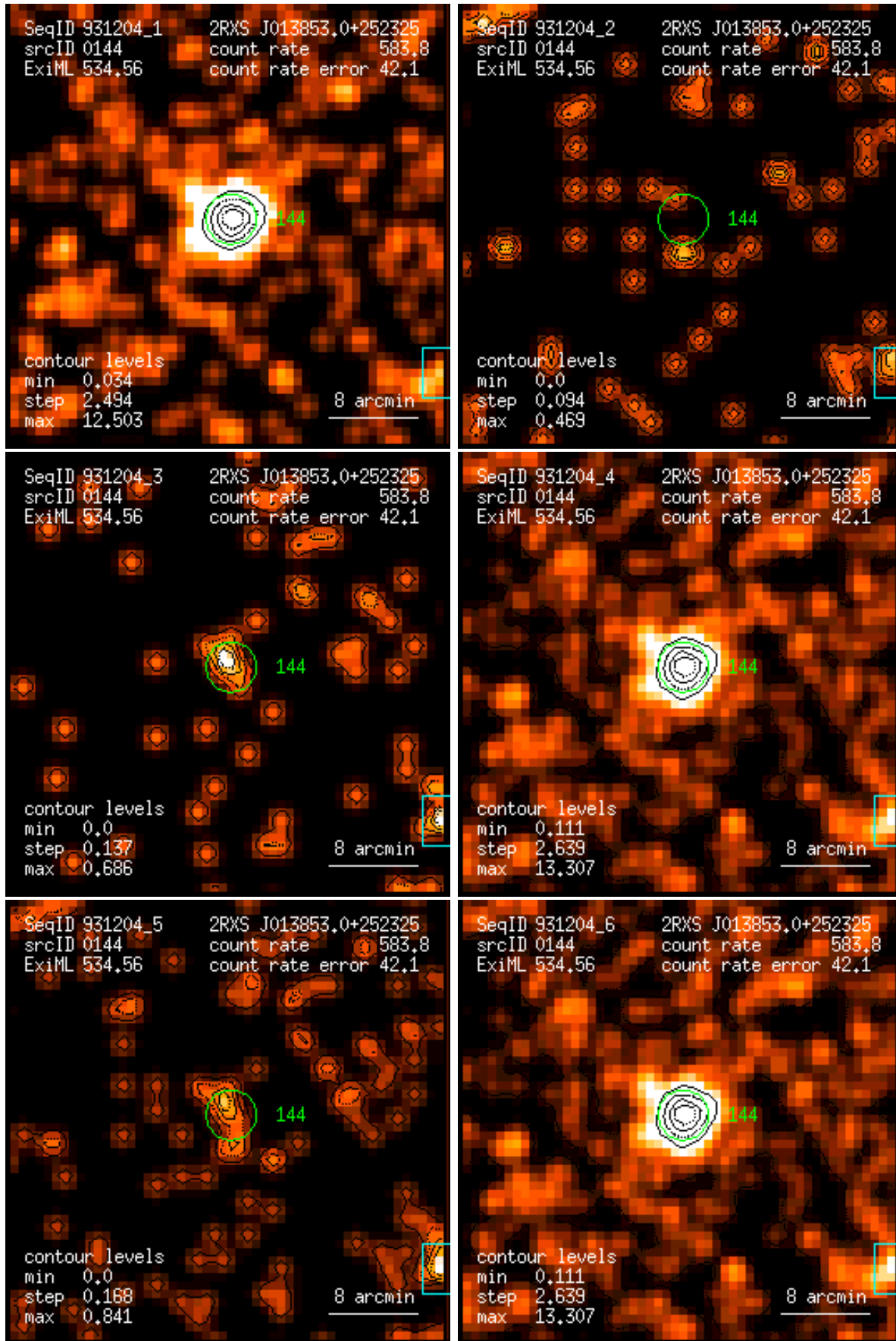
Figure 144: RASS 931204: detection 0144: band rate images, Gaussian filter: (1) PSPC channels 11 – 41, (2) 52 – 90, (3) 91 – 201, (4) 11 – 235, (5) 52 – 201, (6) 11 – 201. Broad band rates in counts/ks. Band rate contour levels in counts/ks/arcmin 2 .
