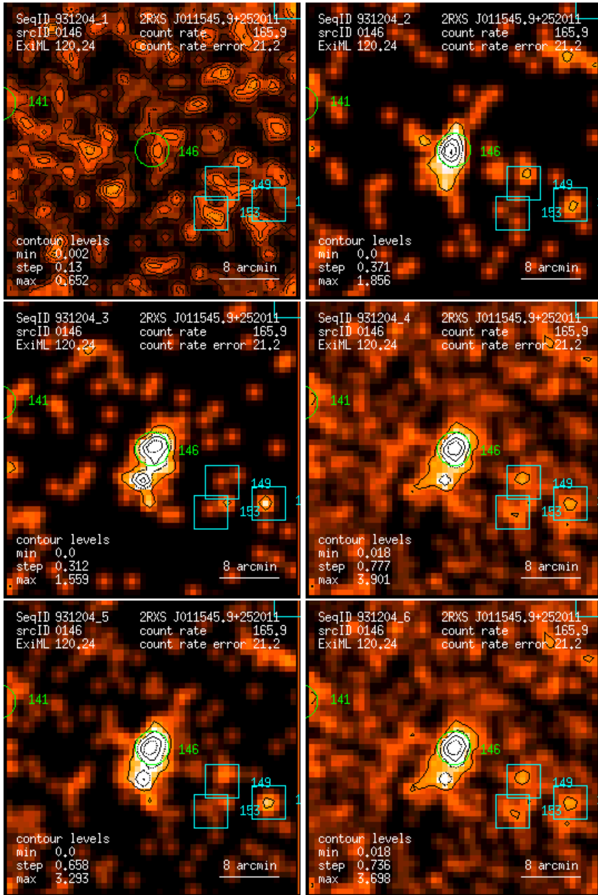
Figure 146: RASS 931204: detection 0146: band rate images, Gaussian filter: (1) PSPC channels 11 – 41, (2) 52 – 90, (3) 91 – 201, (4) 11 – 235, (5) 52 – 201, (6) 11 – 201. Broad band rates in counts/ks. Band rate contour levels in counts/ks/arcmin 2 .
