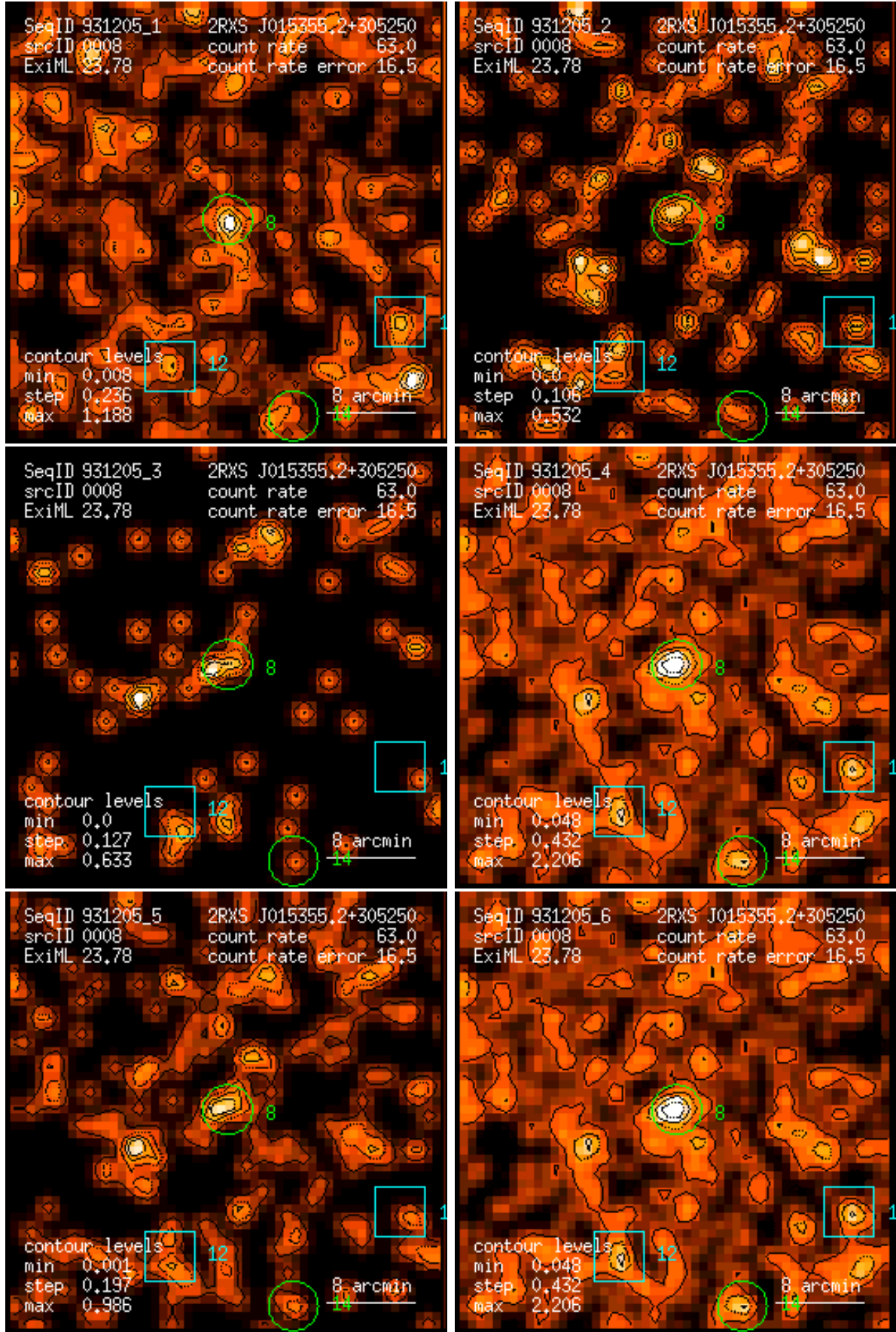
Figure 8: RASS 931205: detection 0008: band rate images, Gaussian filter: (1) PSPC channels 11 – 41, (2) 52 – 90, (3) 91 – 201, (4) 11 – 235, (5) 52 – 201, (6) 11 – 201. Broad band rates in counts/ks. Band rate contour levels in counts/ks/arcmin 2 .
