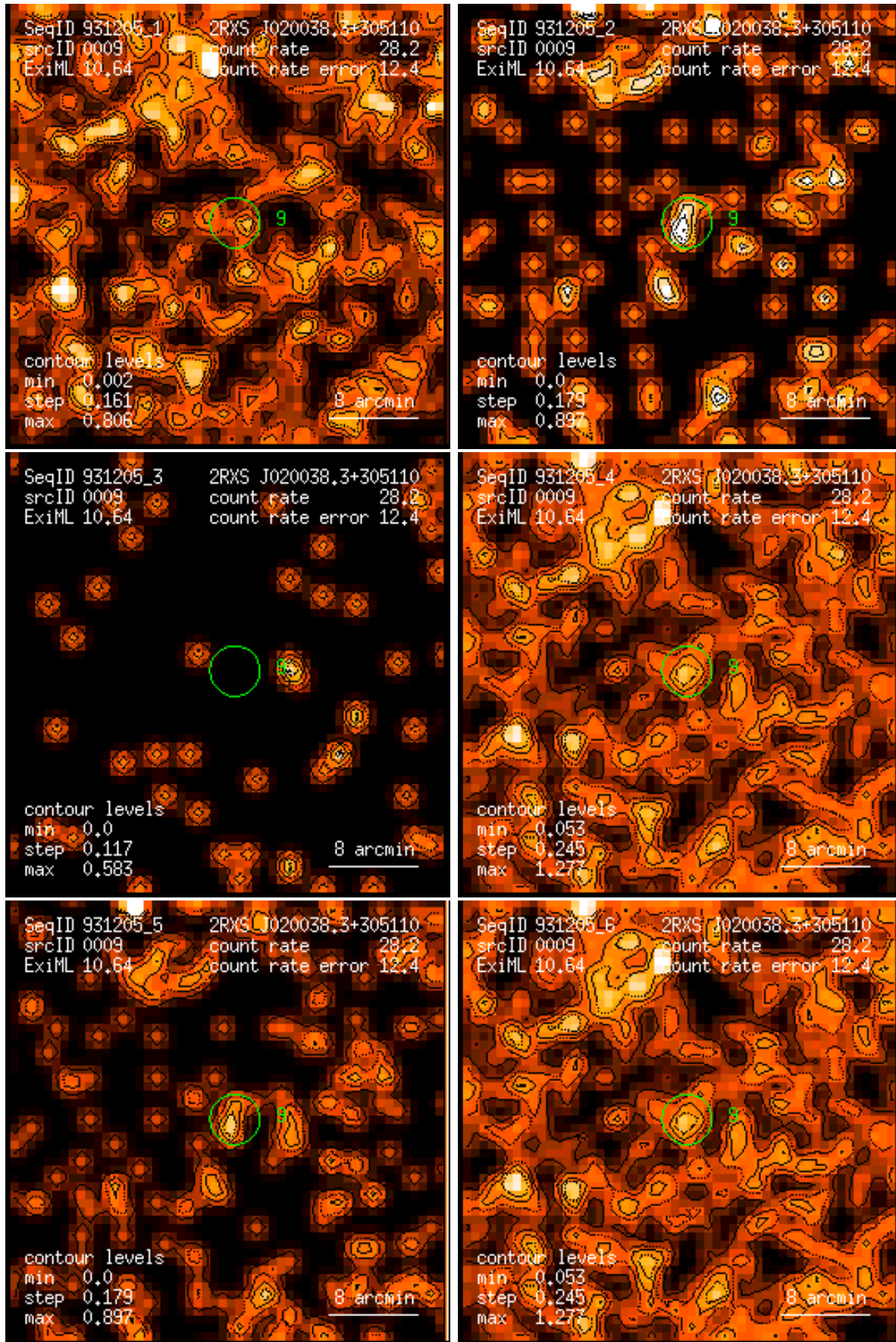
Figure 9: RASS 931205: detection 0009: band rate images, Gaussian filter: (1) PSPC channels 11 – 41, (2) 52 – 90, (3) 91 – 201, (4) 11 – 235, (5) 52 – 201, (6) 11 – 201. Broad band rates in counts/ks. Band rate contour levels in counts/ks/arcmin 2 .
