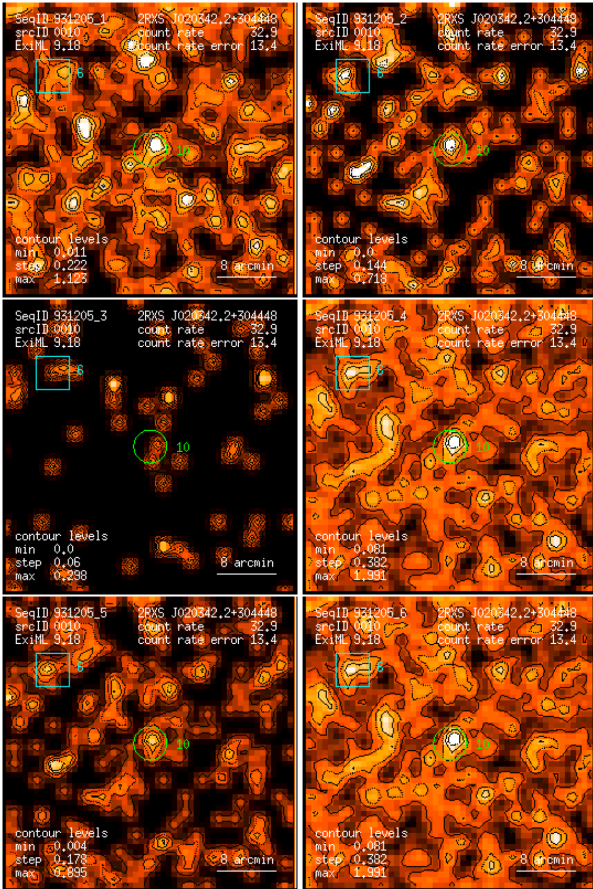
Figure 10: RASS 931205: detection 0010: band rate images, Gaussian filter: (1) PSPC channels 11 – 41, (2) 52 – 90, (3) 91 – 201, (4) 11 – 235, (5) 52 – 201, (6) 11 – 201. Broad band rates in counts/ks. Band rate contour levels in counts/ks/arcmin 2 .
