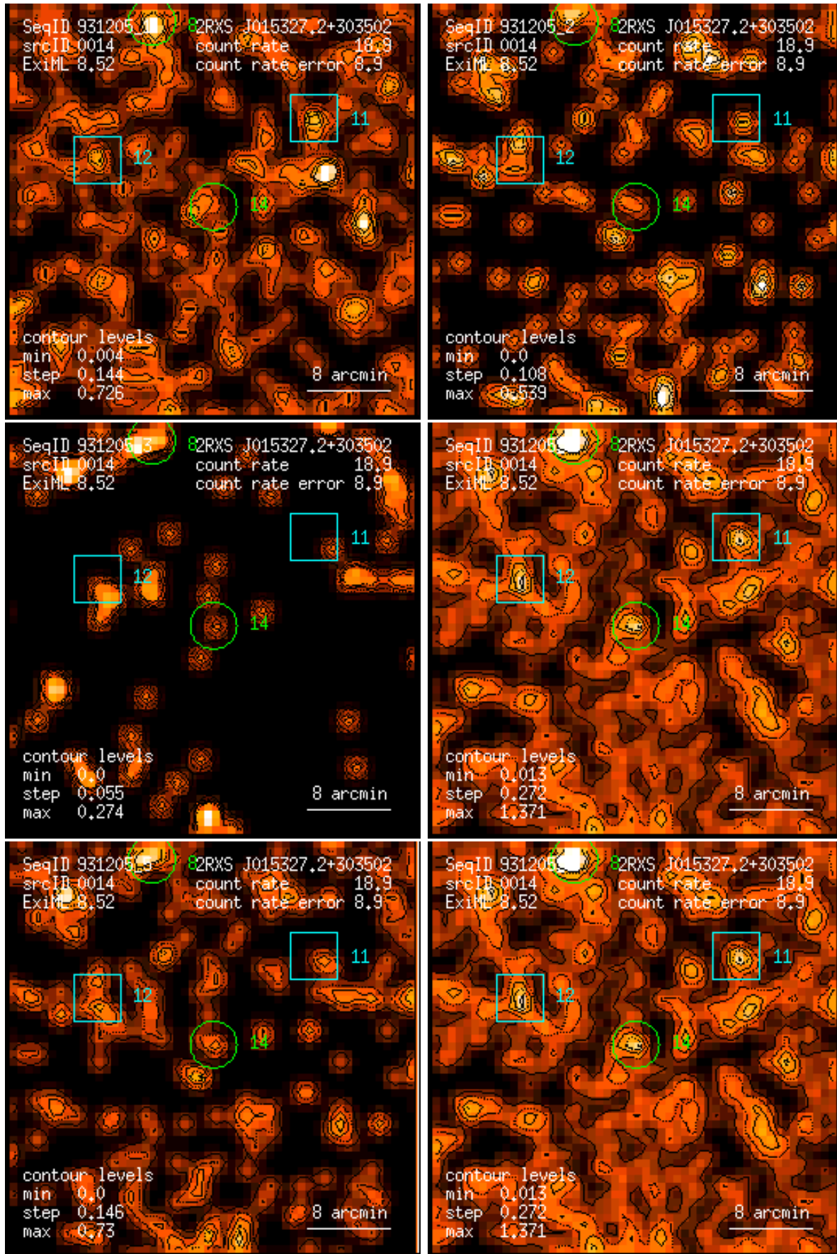
Figure 14: RASS 931205: detection 0014: band rate images, Gaussian filter: (1) PSPC channels 11 – 41, (2) 52 – 90, (3) 91 – 201, (4) 11 – 235, (5) 52 – 201, (6) 11 – 201. Broad band rates in counts/ks. Band rate contour levels in counts/ks/arcmin 2 .
