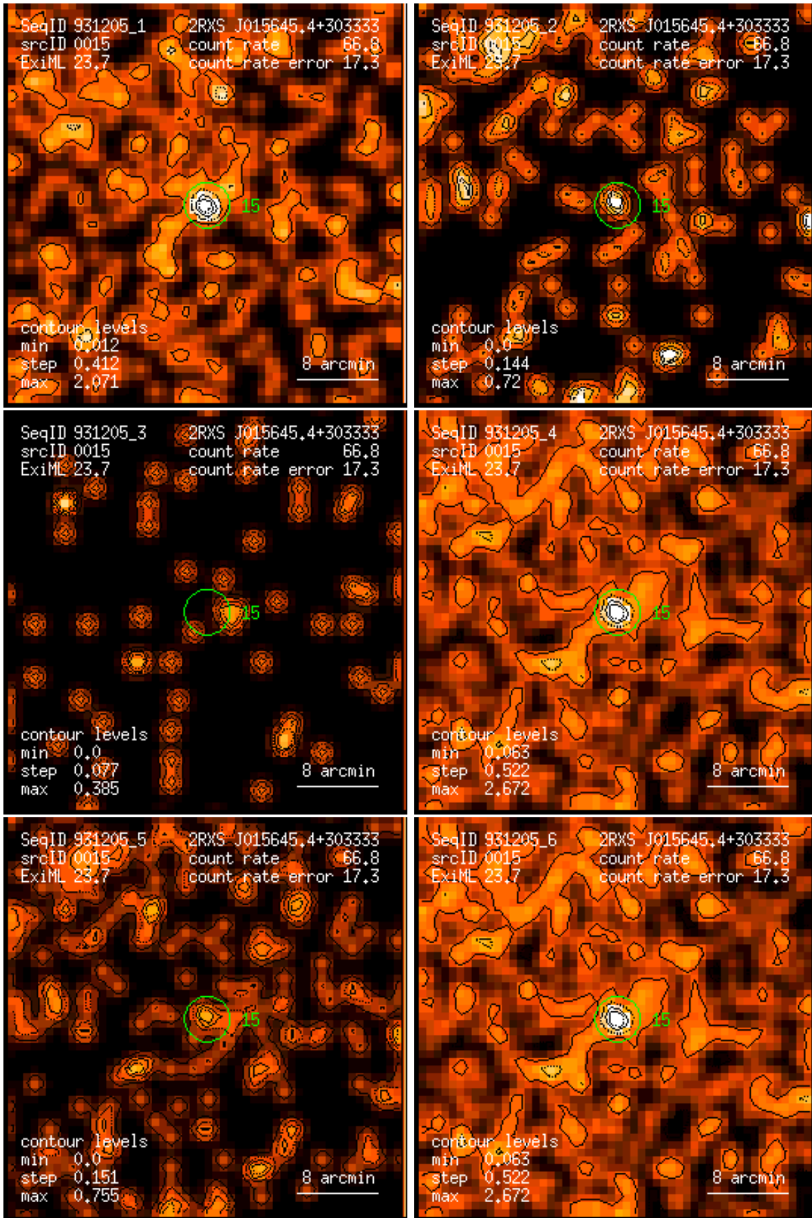
Figure 15: RASS 931205: detection 0015: band rate images, Gaussian filter: (1) PSPC channels 11 – 41, (2) 52 – 90, (3) 91 – 201, (4) 11 – 235, (5) 52 – 201, (6) 11 – 201. Broad band rates in counts/ks. Band rate contour levels in counts/ks/arcmin 2 .
