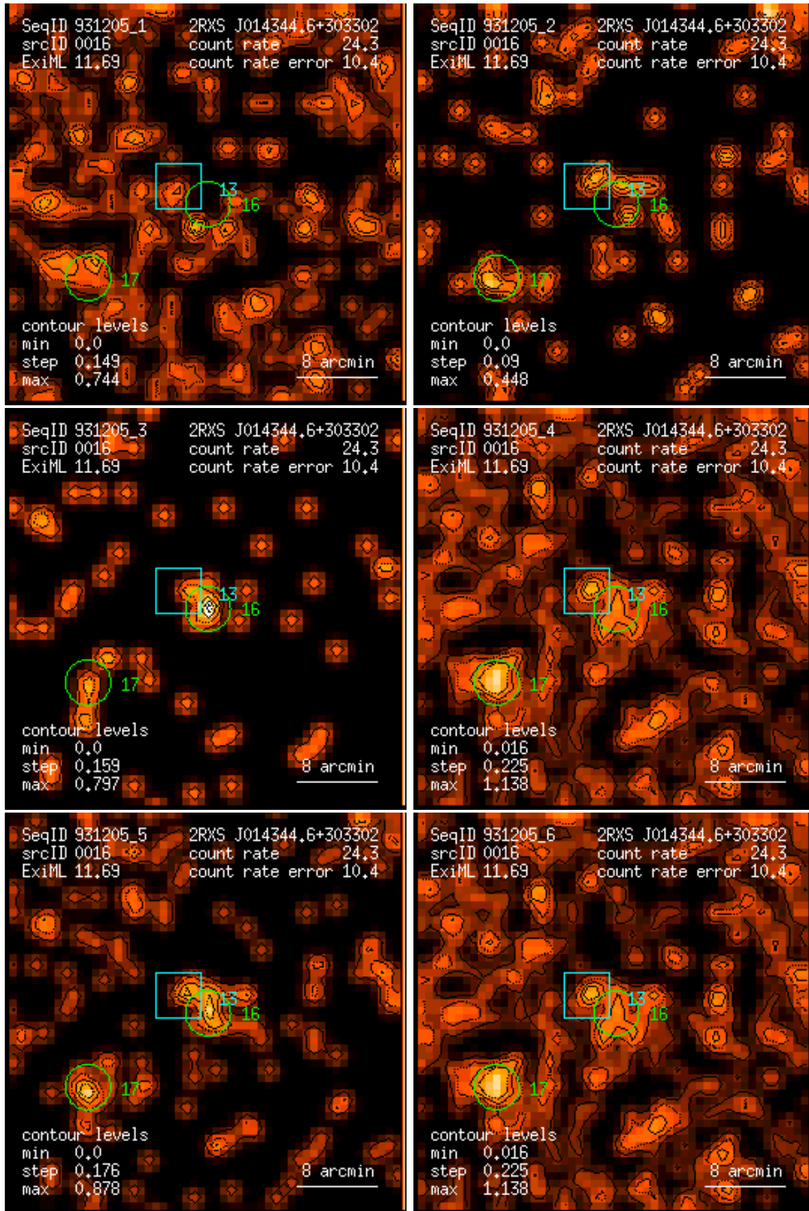
Figure 16: RASS 931205: detection 0016: band rate images, Gaussian filter: (1) PSPC channels 11 – 41, (2) 52 – 90, (3) 91 – 201, (4) 11 – 235, (5) 52 – 201, (6) 11 – 201. Broad band rates in counts/ks. Band rate contour levels in counts/ks/arcmin 2 .
