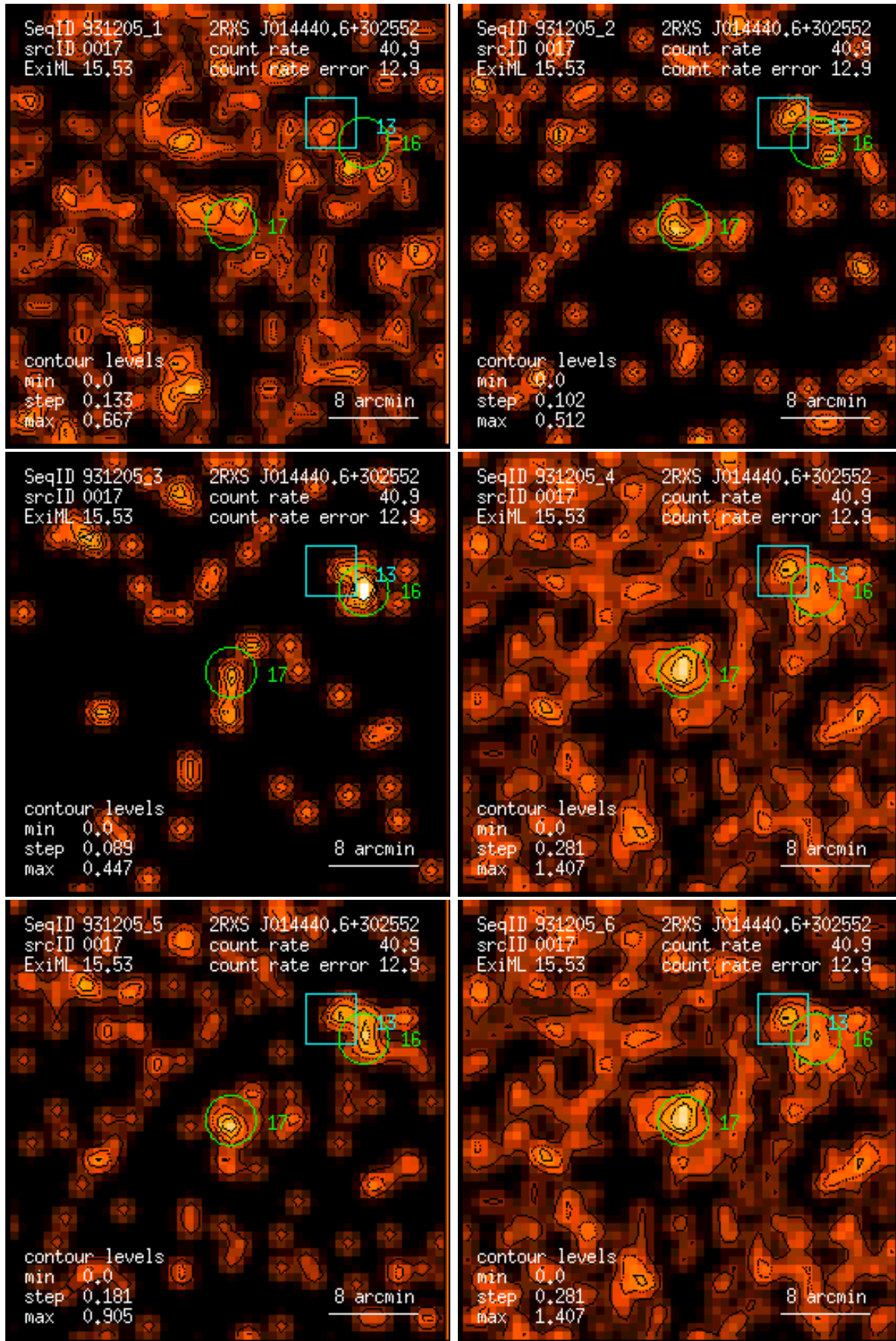
Figure 17: RASS 931205: detection 0017: band rate images, Gaussian filter: (1) PSPC channels 11 – 41, (2) 52 – 90, (3) 91 – 201, (4) 11 – 235, (5) 52 – 201, (6) 11 – 201. Broad band rates in counts/ks. Band rate contour levels in counts/ks/arcmin 2 .
