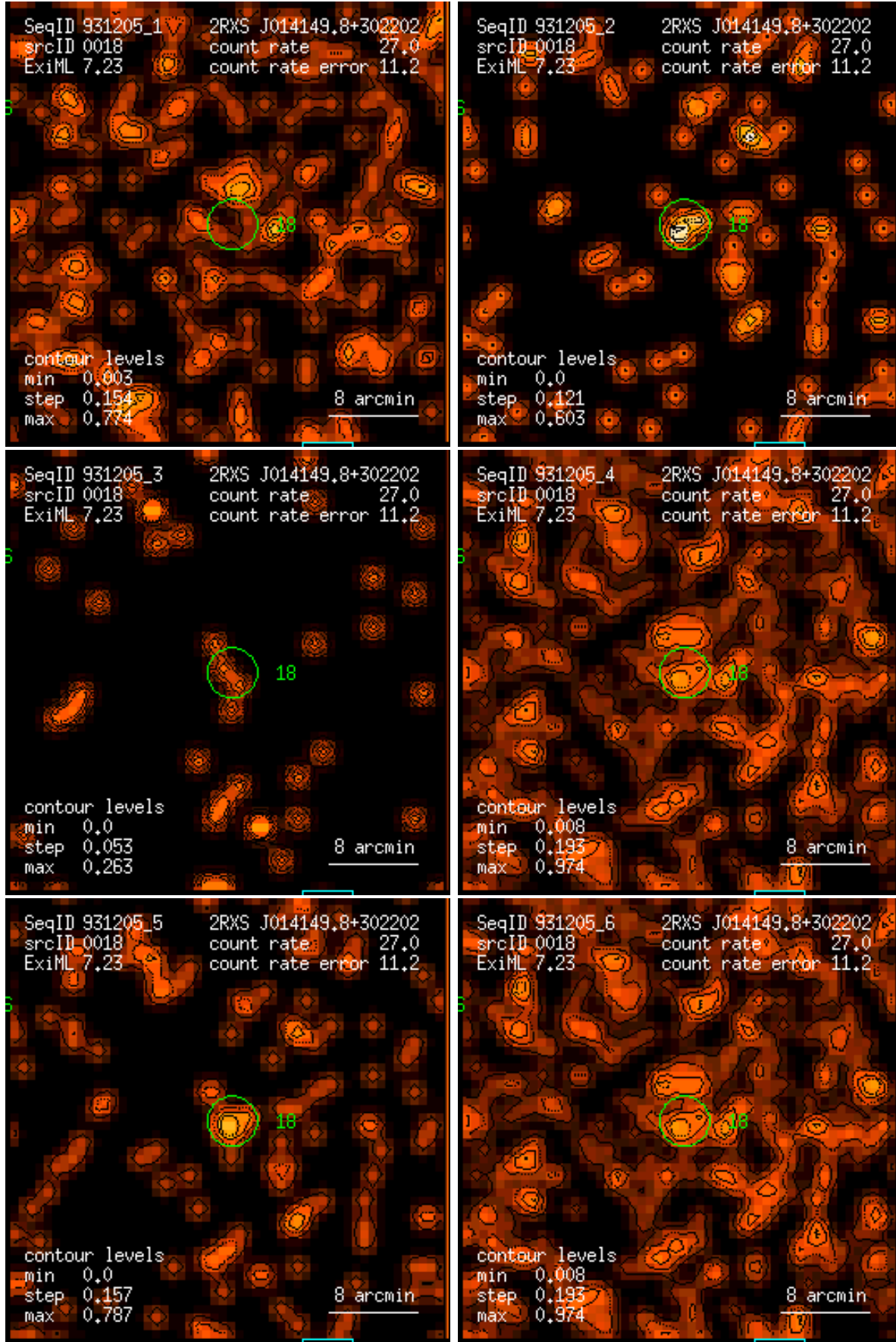
Figure 18: RASS 931205: detection 0018: band rate images, Gaussian filter: (1) PSPC channels 11 – 41, (2) 52 – 90, (3) 91 – 201, (4) 11 – 235, (5) 52 – 201, (6) 11 – 201. Broad band rates in counts/ks. Band rate contour levels in counts/ks/arcmin 2 .
