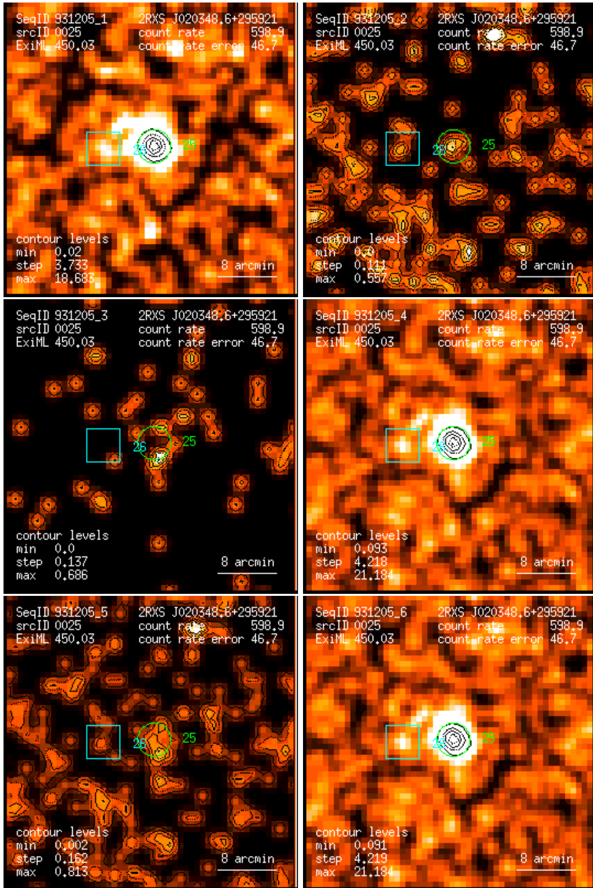
Figure 25: RASS 931205: detection 0025: band rate images, Gaussian filter: (1) PSPC channels 11 – 41, (2) 52 – 90, (3) 91 – 201, (4) 11 – 235, (5) 52 – 201, (6) 11 – 201. Broad band rates in counts/ks. Band rate contour levels in counts/ks/arcmin 2 .
