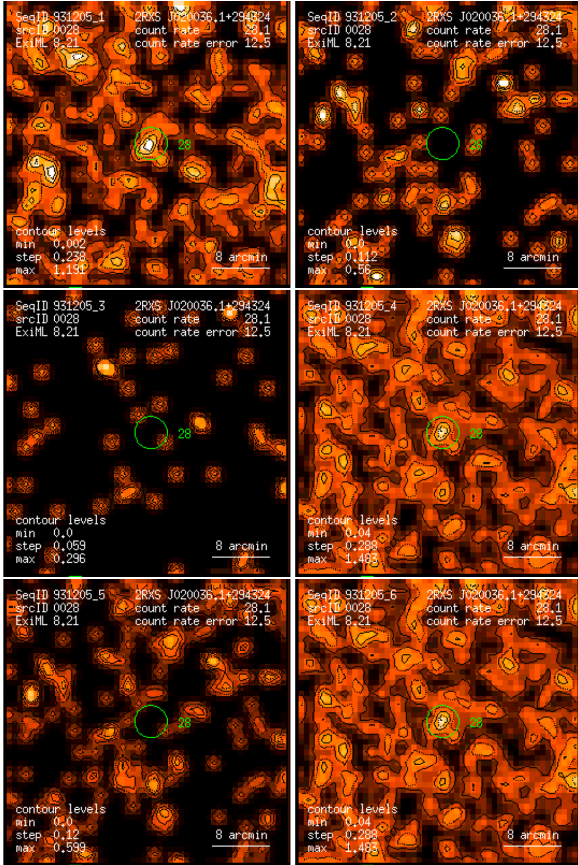
Figure 28: RASS 931205: detection 0028: band rate images, Gaussian filter: (1) PSPC channels 11 – 41, (2) 52 – 90, (3) 91 – 201, (4) 11 – 235, (5) 52 – 201, (6) 11 – 201. Broad band rates in counts/ks. Band rate contour levels in counts/ks/arcmin 2 .
