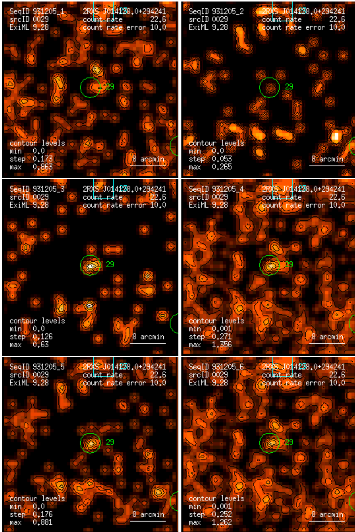
Figure 29: RASS 931205: detection 0029: band rate images, Gaussian filter: (1) PSPC channels 11 – 41, (2) 52 – 90, (3) 91 – 201, (4) 11 – 235, (5) 52 – 201, (6) 11 – 201. Broad band rates in counts/ks. Band rate contour levels in counts/ks/arcmin 2 .
