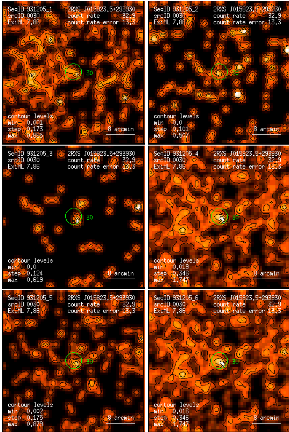
Figure 30: RASS 931205: detection 0030: band rate images, Gaussian filter: (1) PSPC channels 11 – 41, (2) 52 – 90, (3) 91 – 201, (4) 11 – 235, (5) 52 – 201, (6) 11 – 201. Broad band rates in counts/ks. Band rate contour levels in counts/ks/arcmin 2 .
